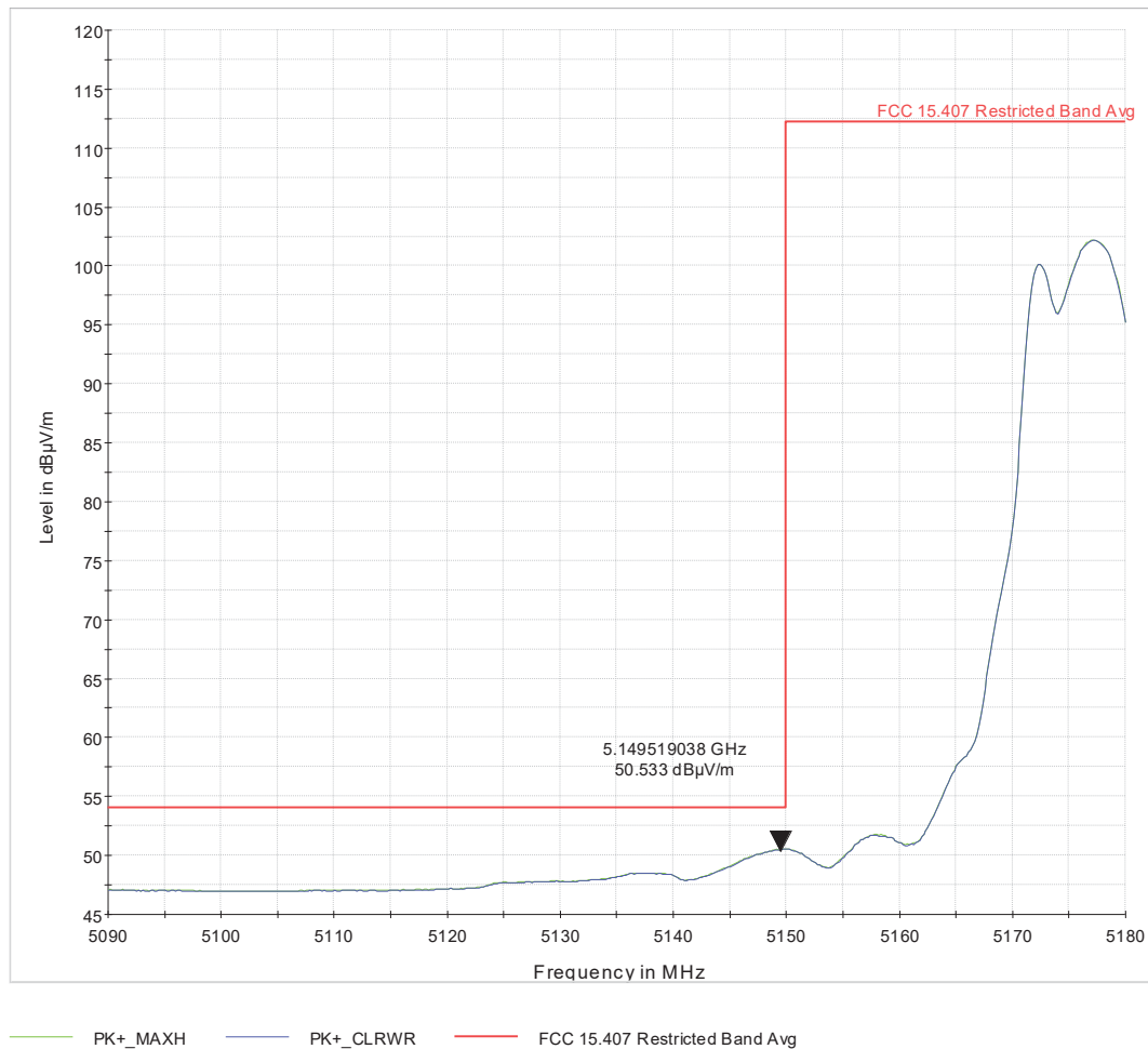
Figure 48: UNII-1 Low Band Edge for 802.11a No HT 6Mbps at 5180 MHz-Average
