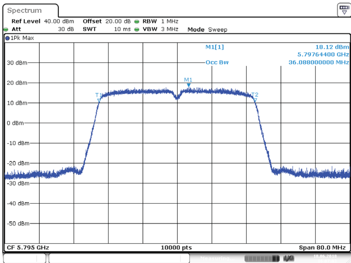
Figure 9: 99% Occupied Bandwidth, Channel 159 at 802.11n HT40+ MCS0, Chain 3
