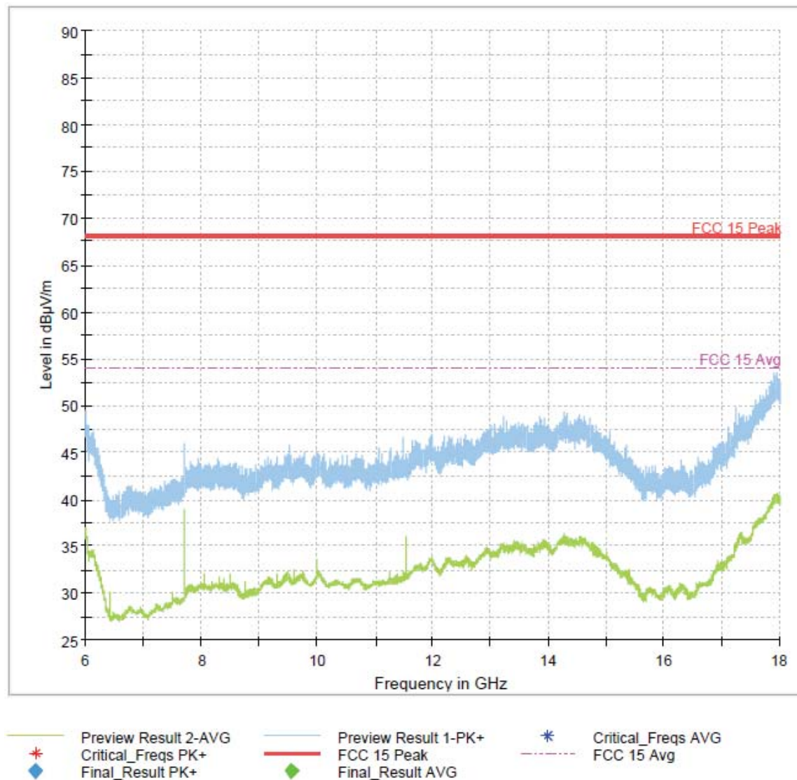
Figure 180: 6-18GHz 802.11ac VHT80 Mode Channel 155
