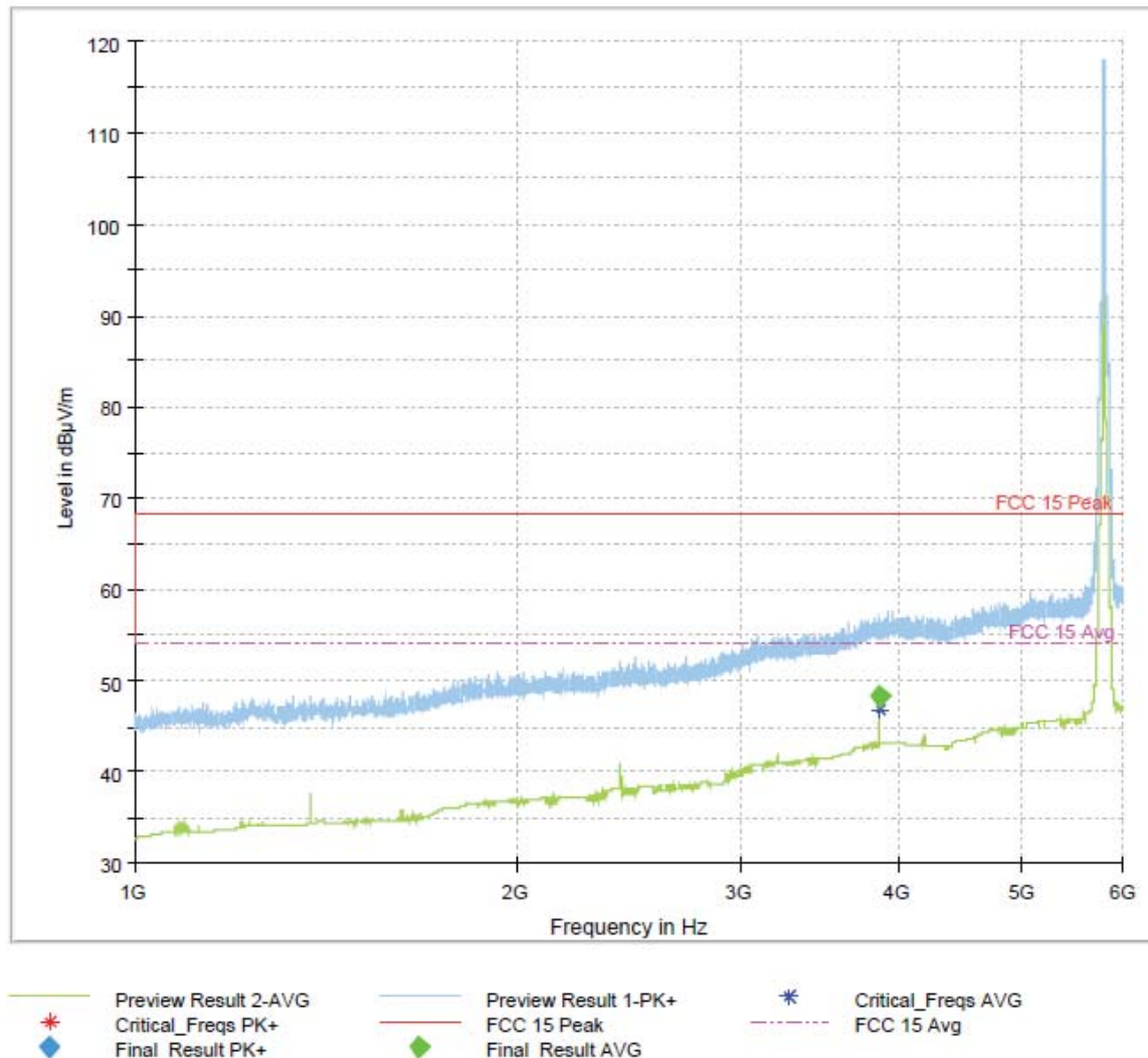
Figure 174: 1-6GHz 802.11ac VHT40 Mode Channel 159
