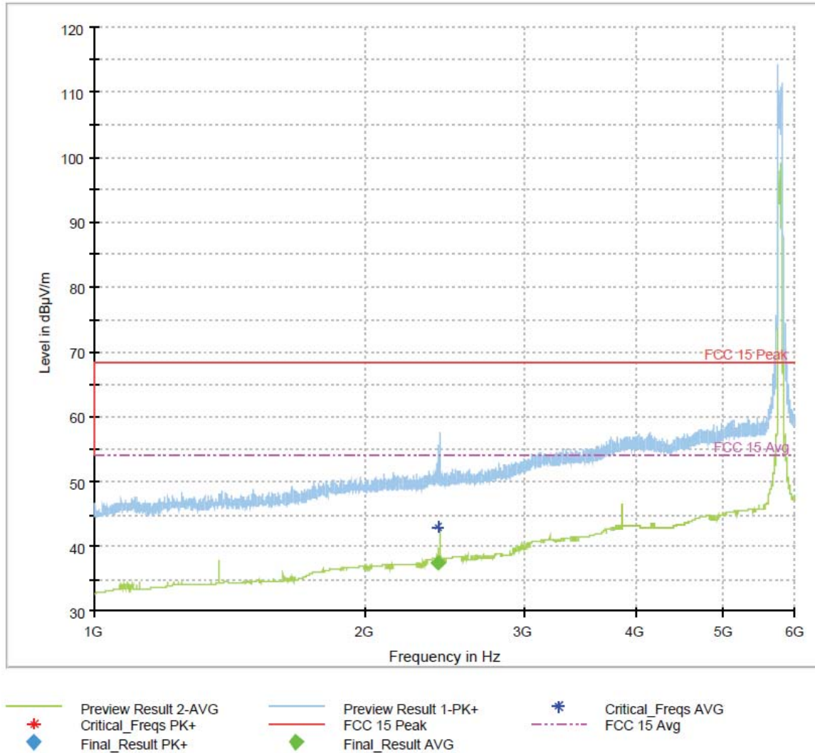
Figure 179: 1-6GHz 802.11ac VHT80 Mode Channel 155
