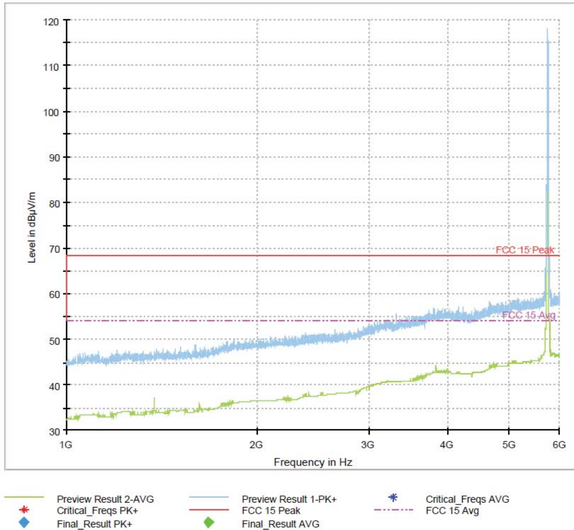
Figure 164: 1-6GHz 802.11ac VHT20 Mode Channel 149
