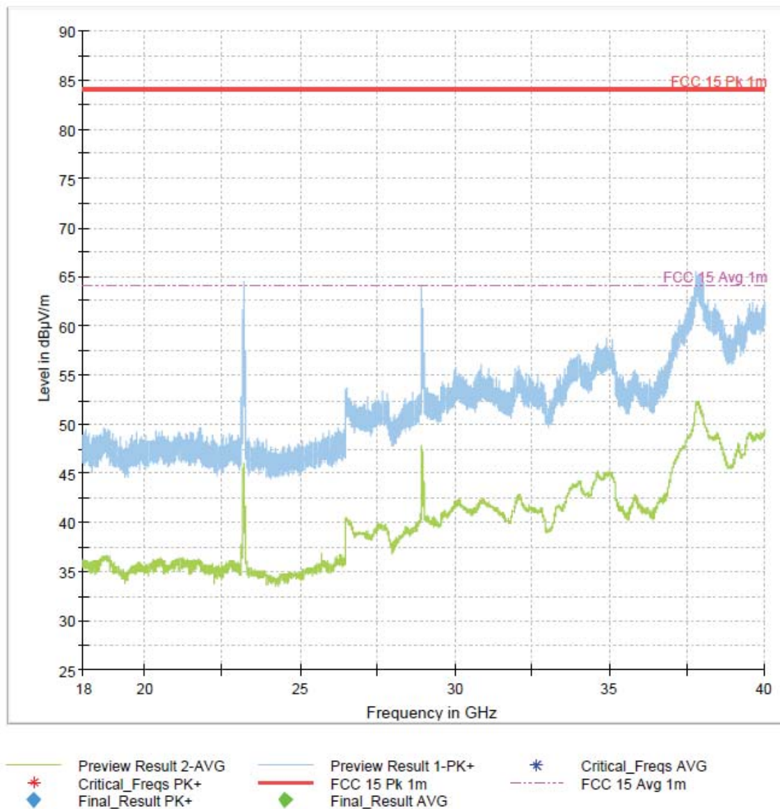
Figure 178: 18-40GHz 802.11ac VHT40 Mode Channel 159
