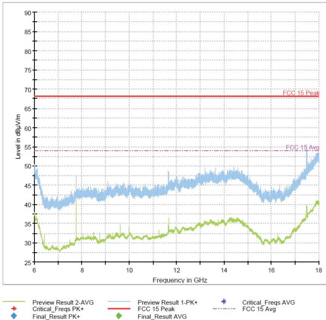
Figure 169: 6-18GHz 802.11ac VHT20 Mode Channel 165
