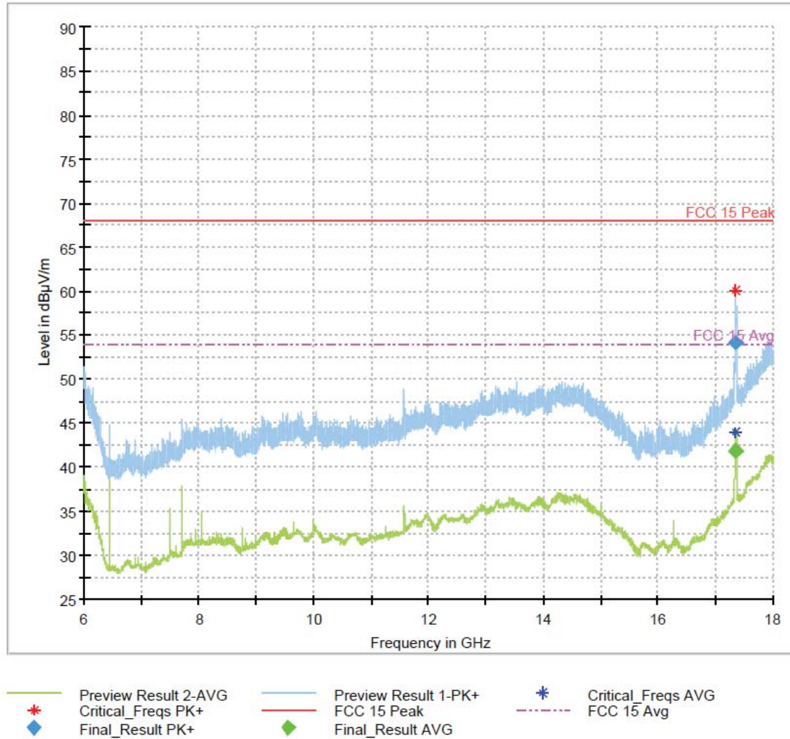
Figure 168: 6-18GHz 802.11ac VHT20 Mode Channel 157
