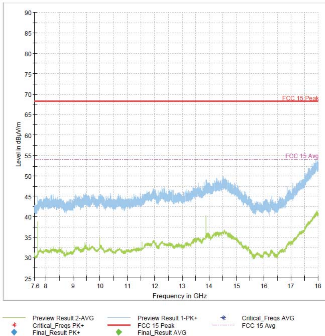
Figure 184: 7.6-18GHz 802.11ac VHT80+80 Mode Channel 42 & 155
