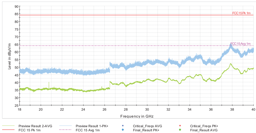
Figure 159: 18-40GHz 802.11ac VHT40 Mode Channel 38
