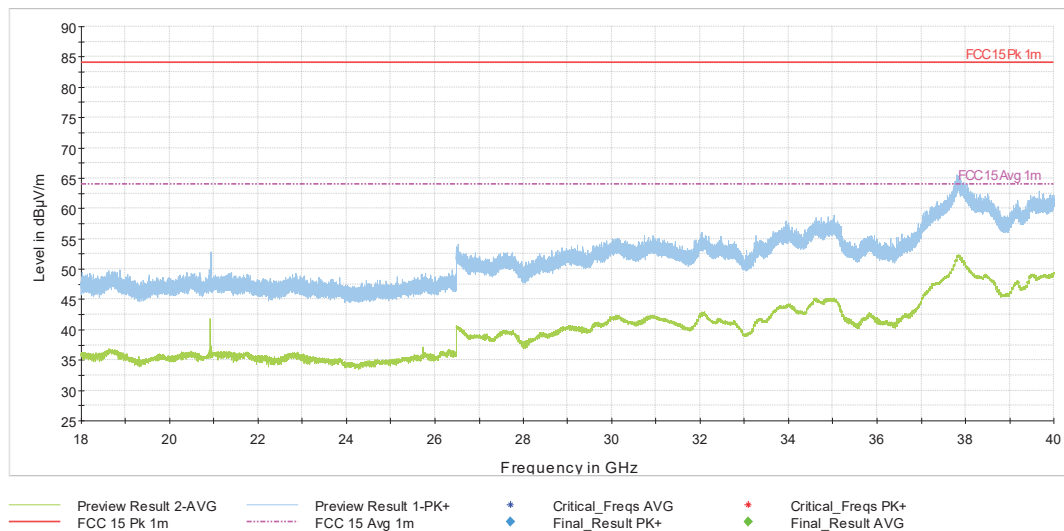
Figure 160: 18-40GHz 802.11ac VHT40 Mode Channel 46
