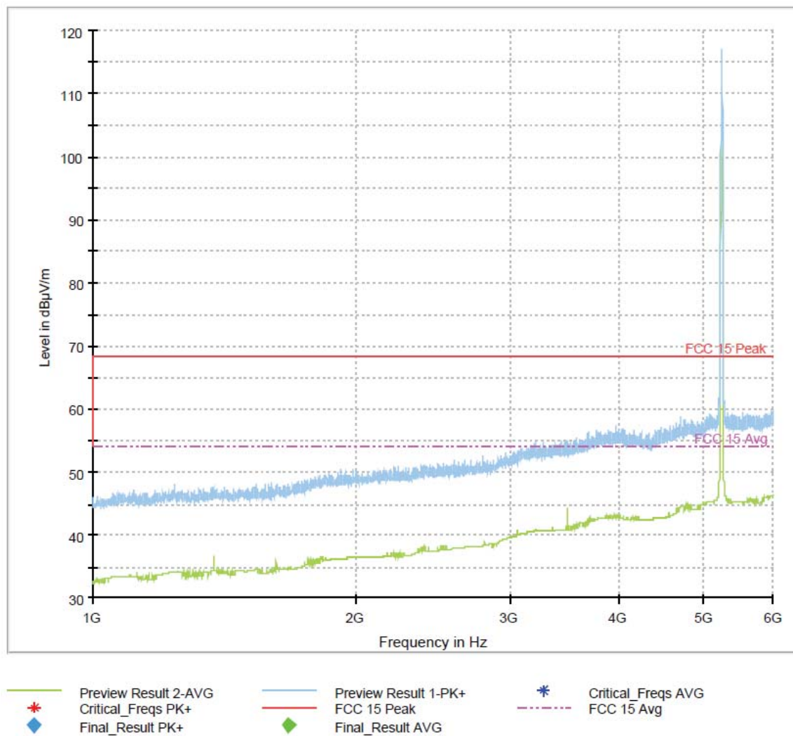
Figure 148: 1-6GHz 802.11ac VHT20 Mode Channel 48
