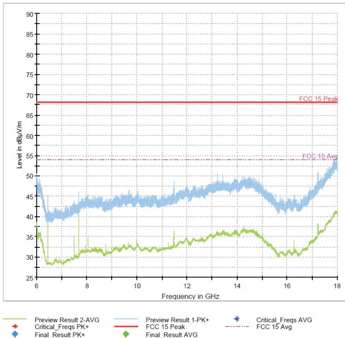
Figure 167: 6-18GHz 802.11ac VHT20 Mode Channel 149
