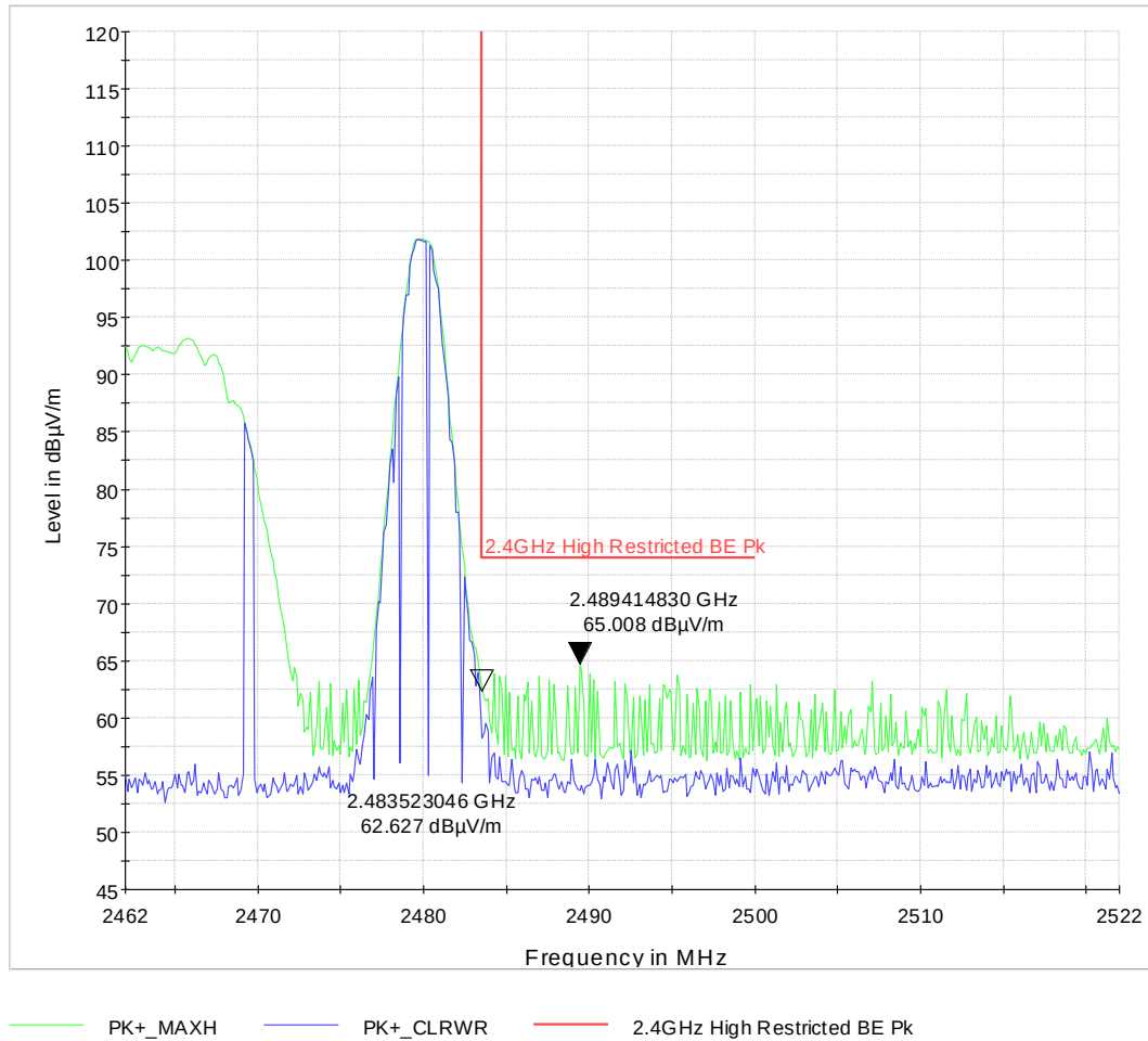
Figure 10: High Channel Restricted Band Edge Peak Detector– BT LE
