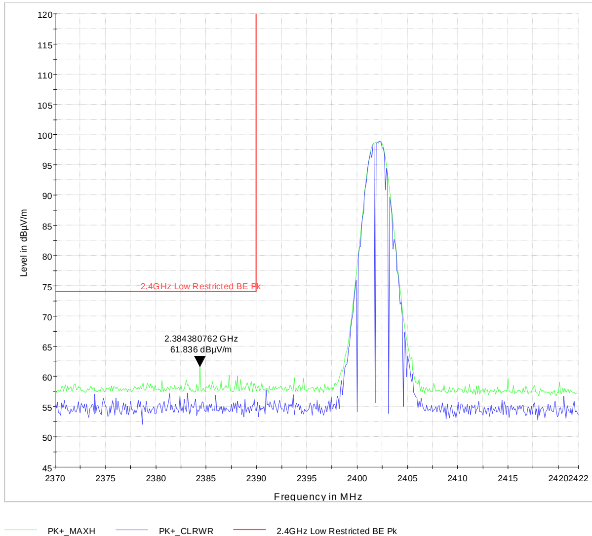
Figure 8: Low Channel Restricted Band Edge Peak Detector– BT LE
