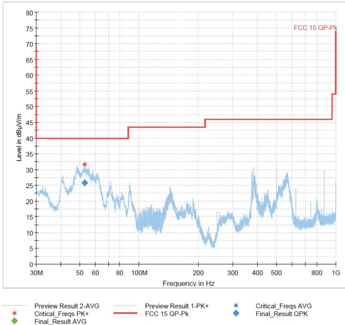
Figure 84: 30MHz-1GHz 802.11n HT20 Mode Channel 1
