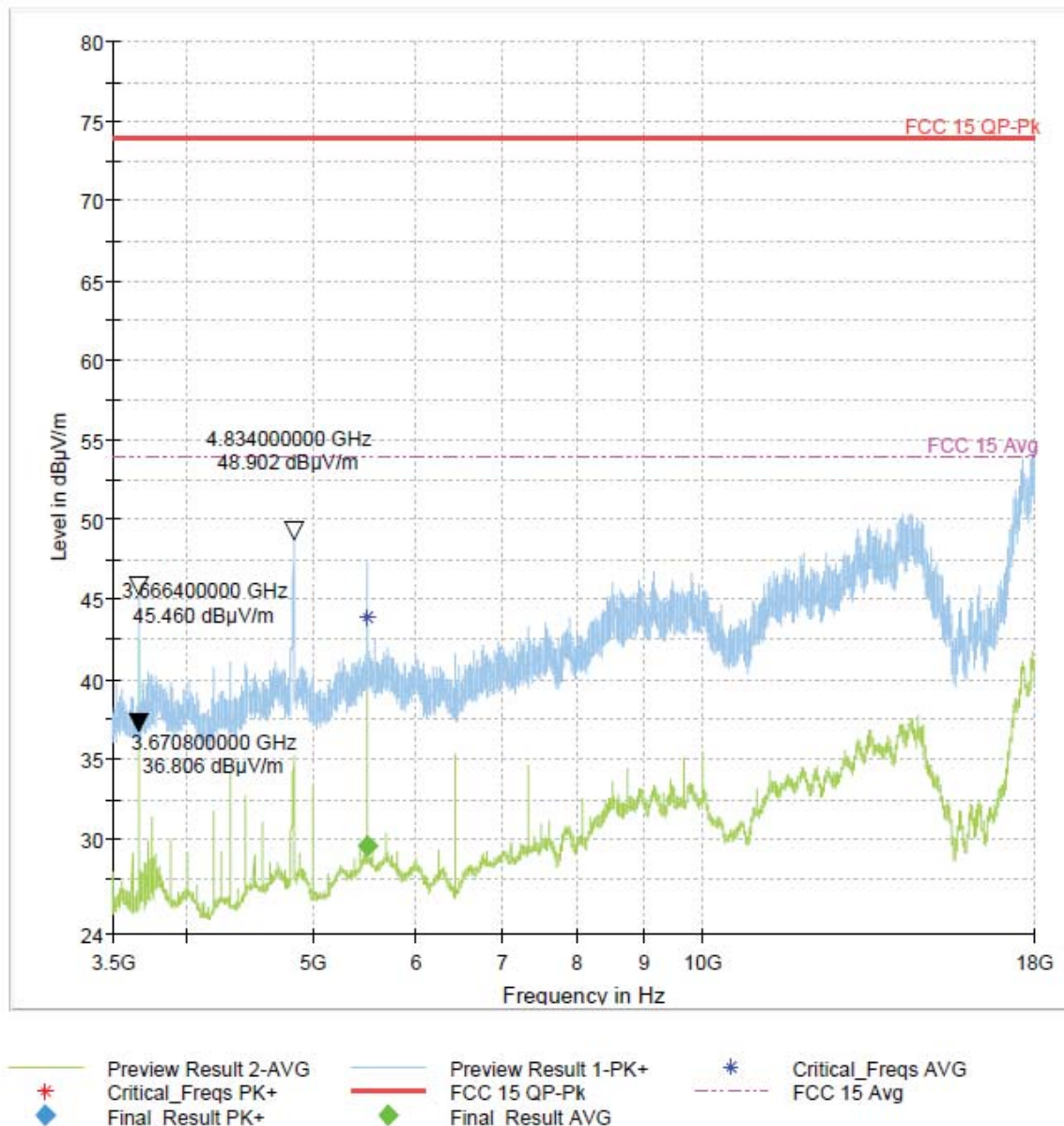
Figure 90: 3.5-18GHz 802.11n HT20 Mode Channel 1
