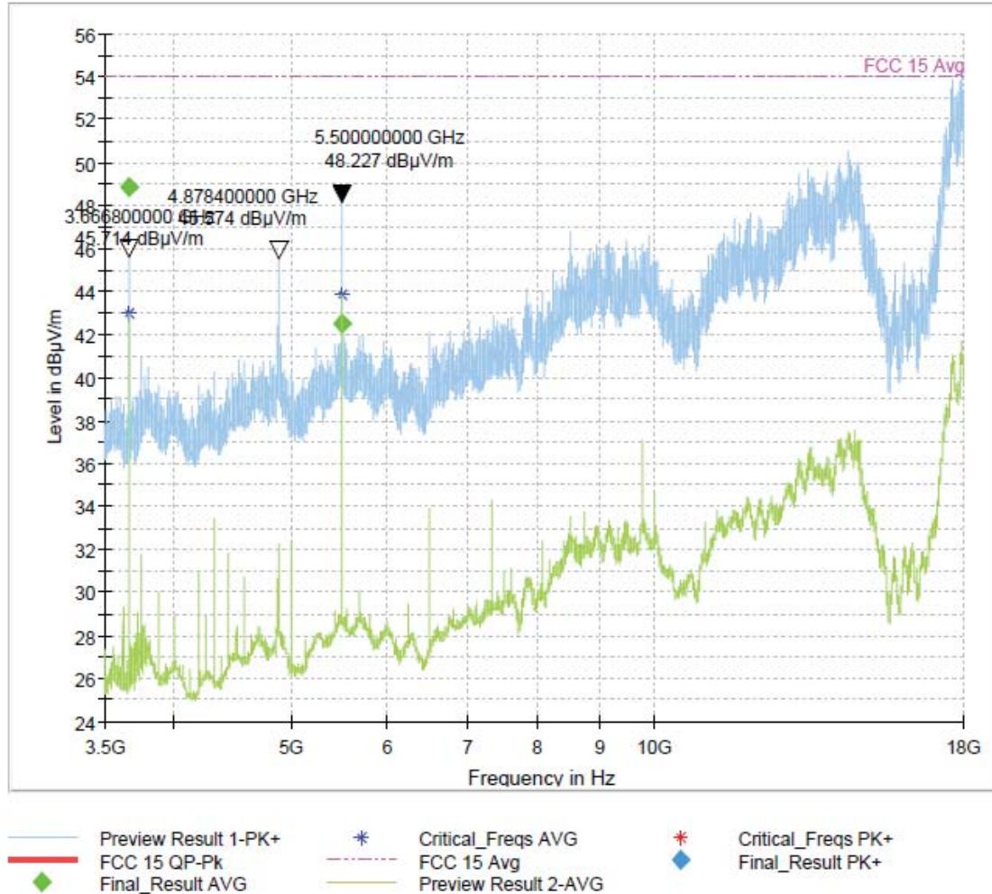
Figure 91: 3.5-18GHz 802.11n HT20 Mode Channel 6
