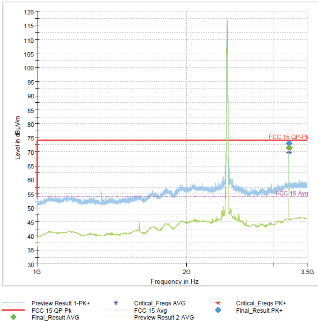
Figure 72: 1-3.5GHz 802.11b Mode Channel 1
