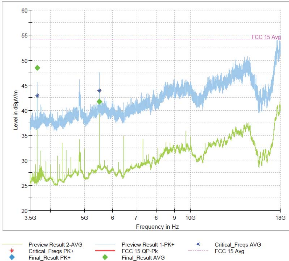
Figure 99: 3.5-18GHz 802.11n HT20 Mode Channel 3
