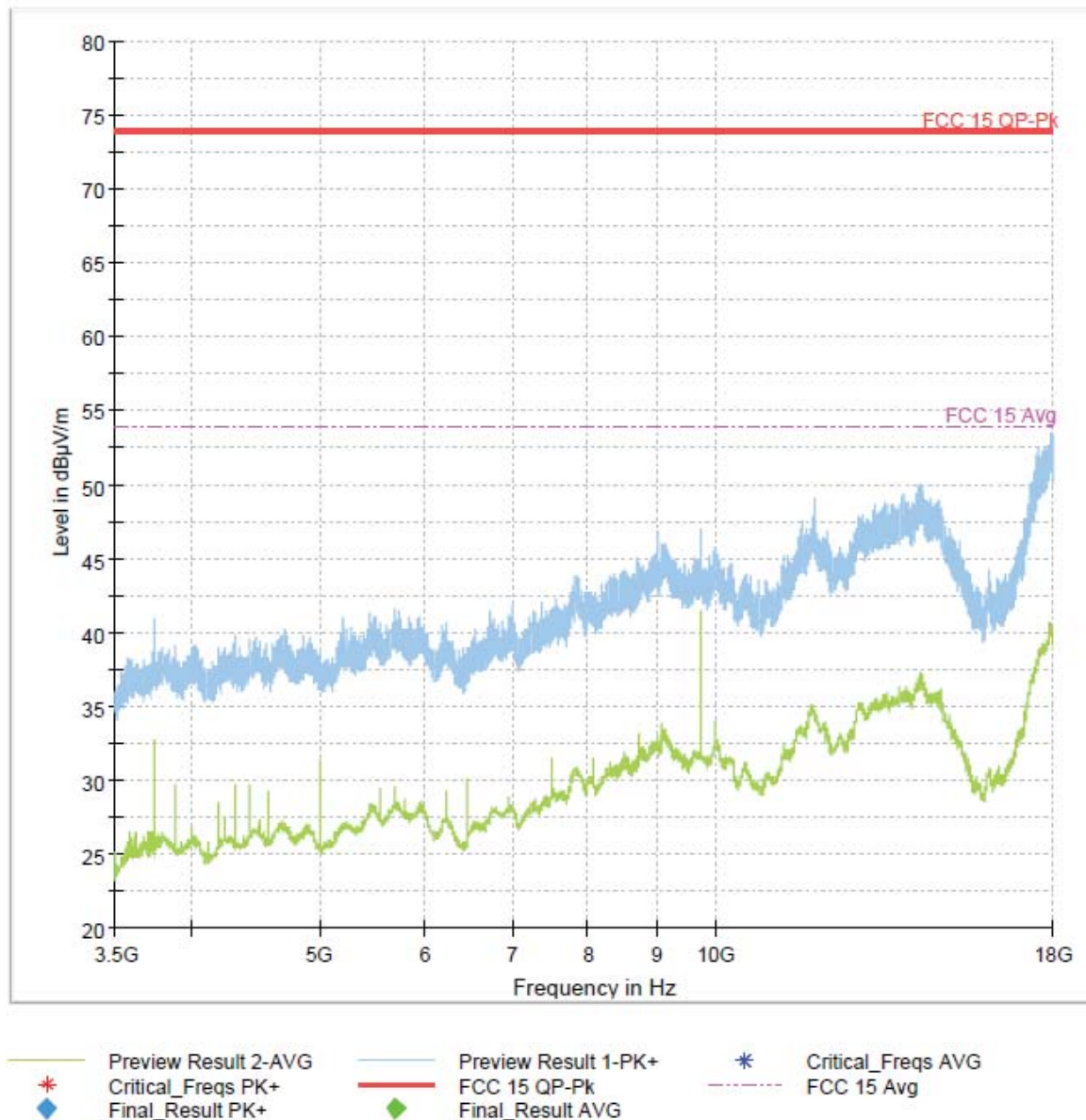
Figure 111: 3.5-18GHz 802.11ac VHT40 Mode Channel 3
