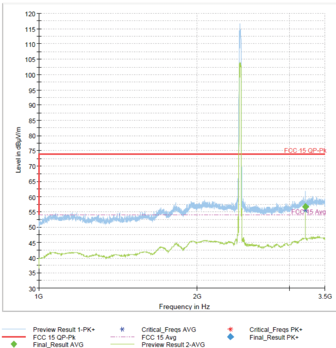
Figure 101: 1-3.5GHz 802.11ac VHT20 Mode Channel 1
