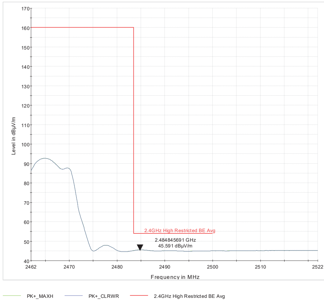
Figure 60: High Band Edge (restricted) for 802.11n HT40 MCS0 at 2452 MHz-Average
