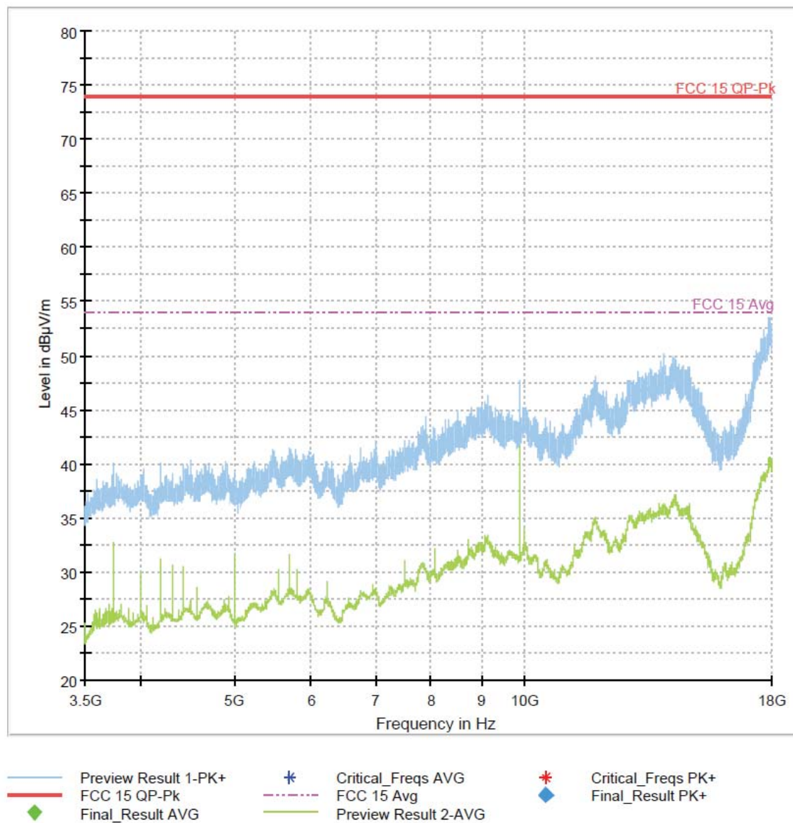
Figure 106: 3.5-18GHz 802.11ac VHT20 Mode Channel 11
