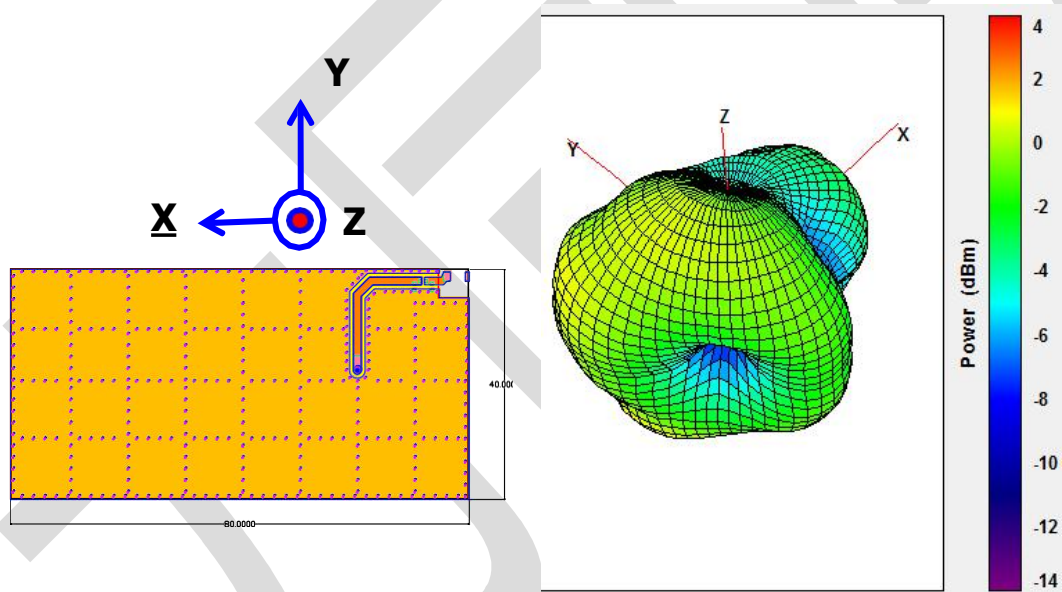
Radiation Pattern
