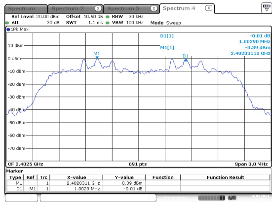
8DPSK_Low_3DH1
