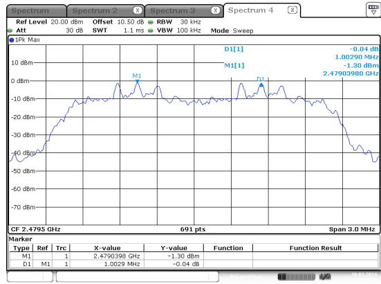
8DPSK_High_3DH1
