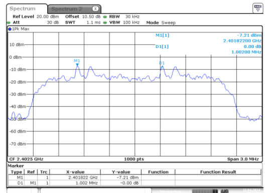
PI/4-DQPSK_Low_2DH1
