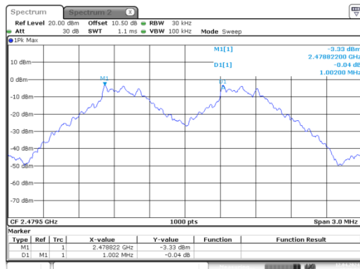
GFSK_High_DH1
