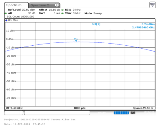
PI/4-DQPSK_High_2DH1
