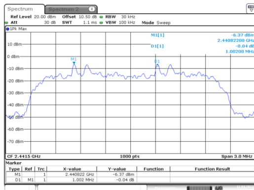
PI/4-DQPSK_Mid_2DH1
