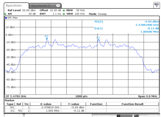
PI/4-DQPSK_High_2DH1
