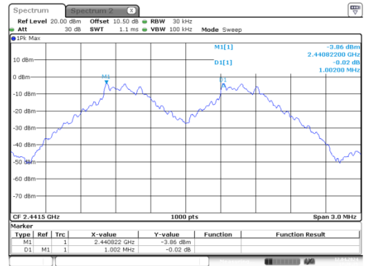
GFSK_Mid_DH1
