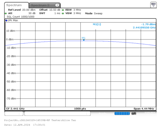
GFSK_Mid_DH1
