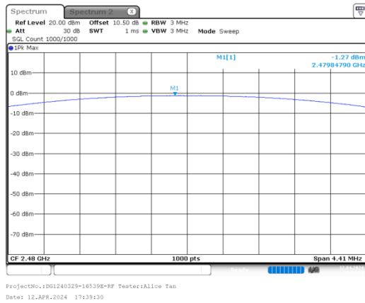
GFSK_High_DH1
