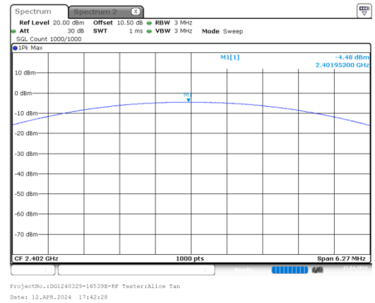
PI/4-DQPSK_Low_2DH1
