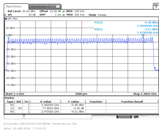
PI/4-DQPSK_Hopping_2DH1
