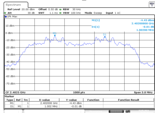
8DPSK_Low
