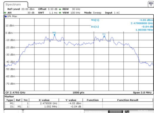
8DPSK_High
