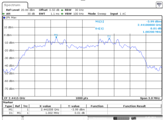
8DPSK_Middle
