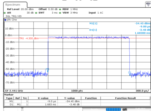
8DPSK_Hopping_3DH3
