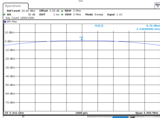
GFSK_Middle
