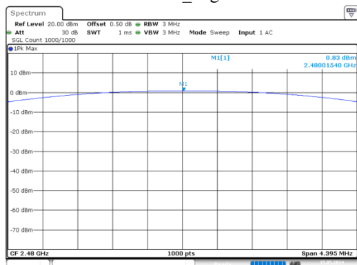
GFSK_High
