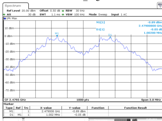
GFSK_High
