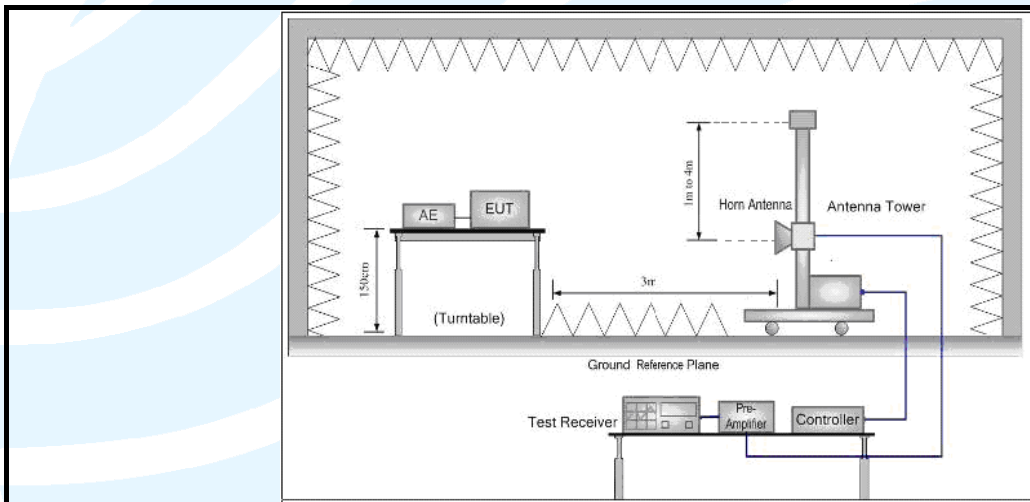
Figure 3. Above 1GHz
