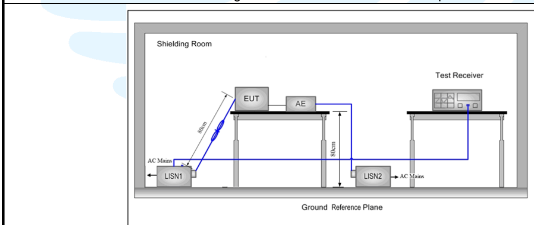
Figure 3. Conducted Emissions setup
