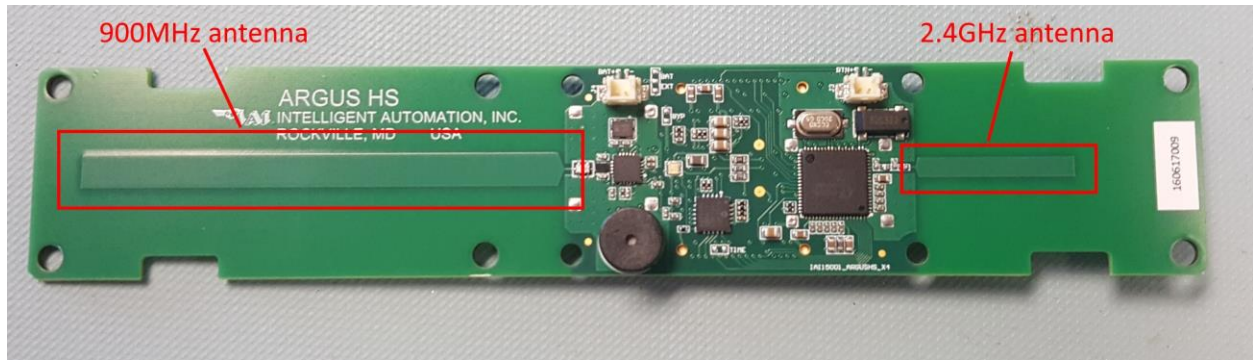
PCB Top Photo with Antennas Noted
