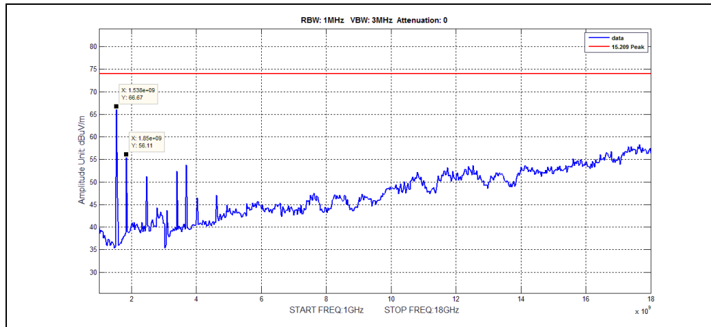
Plot 52. Spurious Emissions, 2.4 GHz, High 900 MHz, High Channel, 1 GHz – 18 GHz, Peak 2.4ghz high 900mhz high channel 1-18ghz peak
