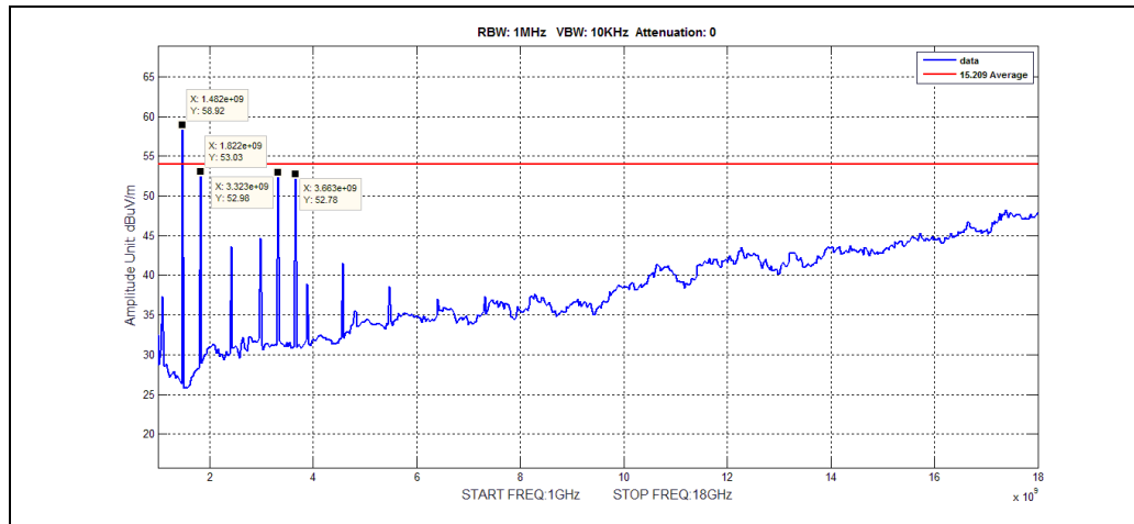
Plot 37. Spurious Emissions, 2.4 GHz, Low 900 MHz, Mid Channel, 1 GHz – 18 GHz, Average
