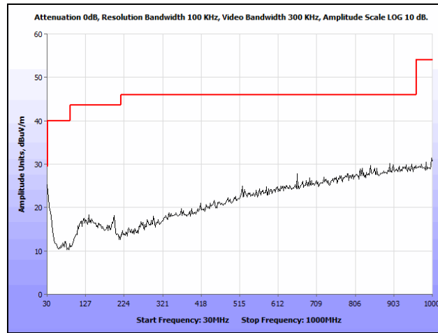
Plot 19. Radiated Spurious Emissions, 30 MHz – 1 GHz, High Channel
