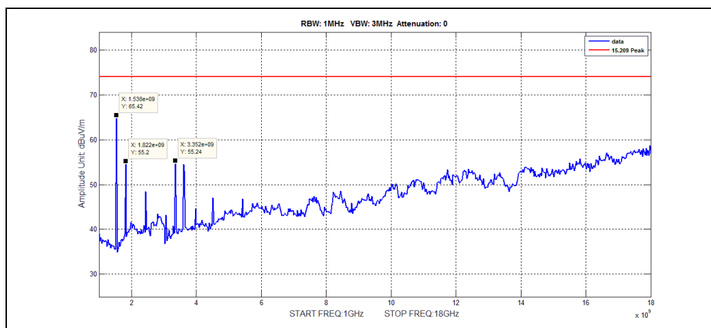
Plot 42. Spurious Emissions, 2.4 GHz, Mid 900 MHz, Low Channel, 1 GHz – 18 GHz, Peak
