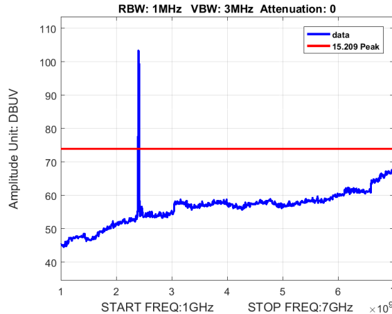
Plot 17. Peak Radiated Spurious Emissions up to 10 th Harmonic, 1-7GHz, Ch. Low
