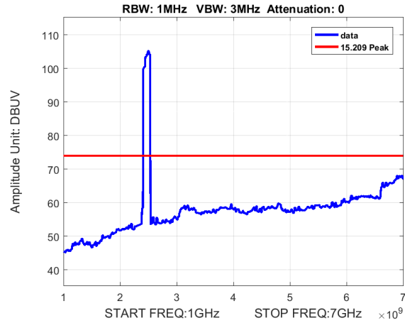
Plot 21. Peak Radiated Spurious Emissions up to 10 th Harmonic, 1-7GHz, Hopping
