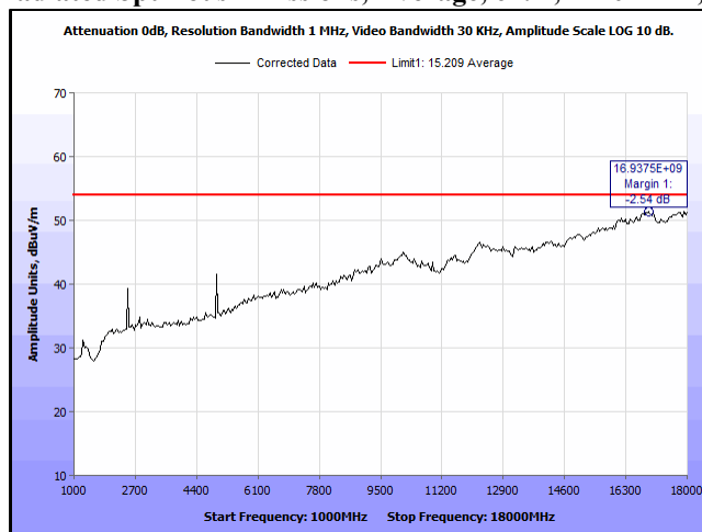
Plot 15. Radiated Spurious Emissions, Average, ch. 14, 2475 MHz, 1 – 18 GHz
