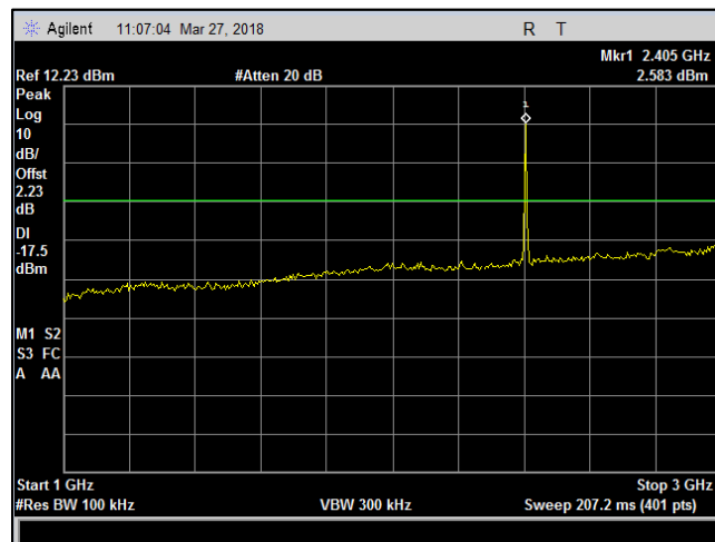
Plot 34. Radiated Spurious Emissions, Ch. 0, 100 kHz, RBW 1 – 3 GHz
