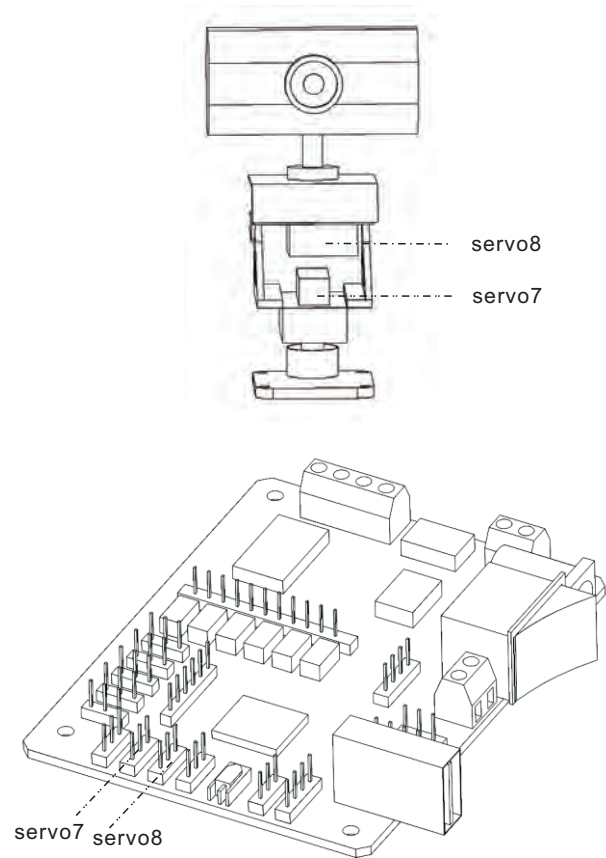
The connection of cradle with 51duino main board
