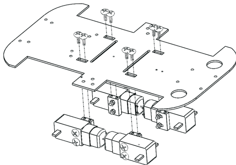
Motor installation
