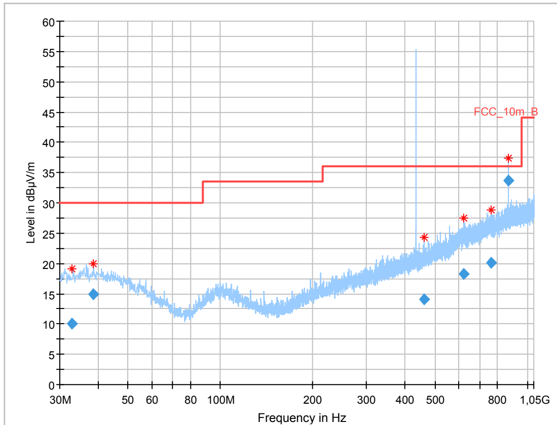
Plot 2: 30 MHz to 1000 MHz, vertical &amp; horizontal polarization
