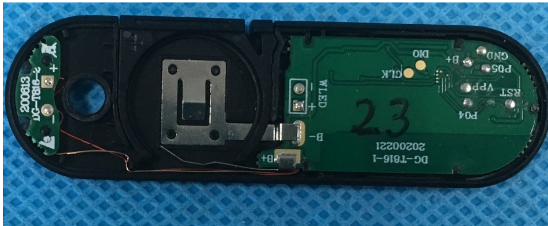
Inner Circuit Bottom View
