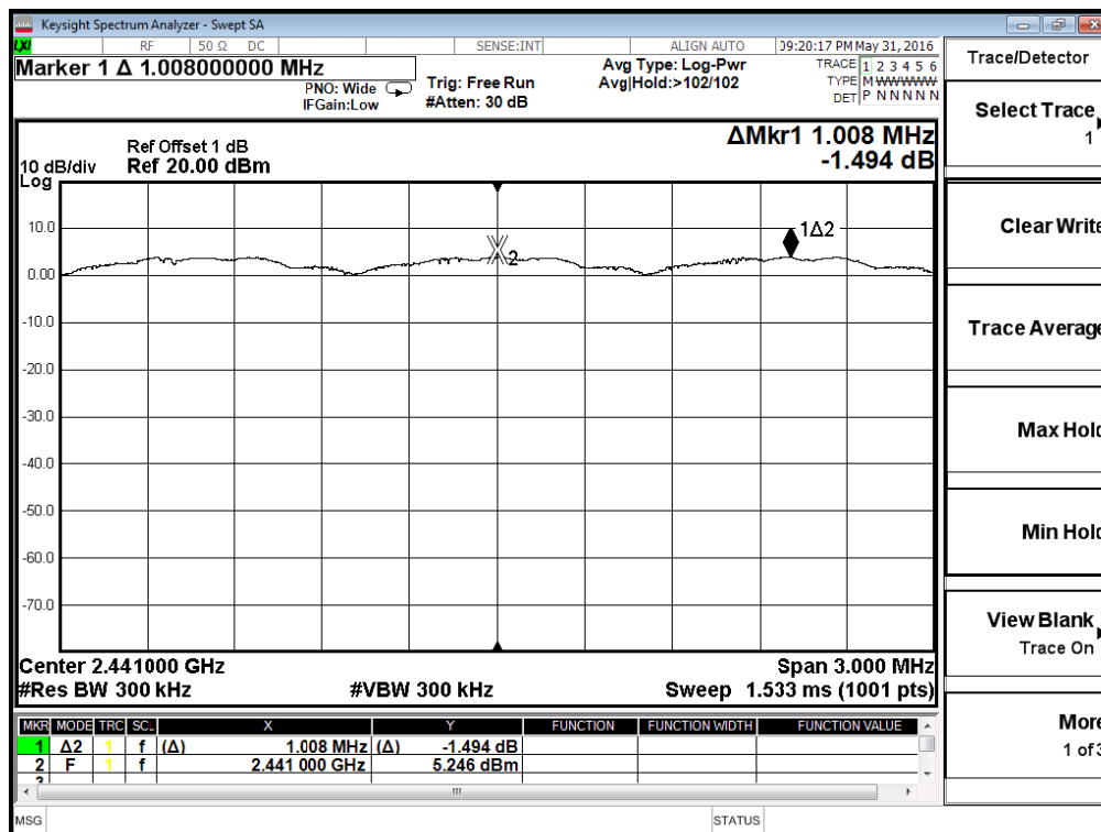
8-DPSK Mode
