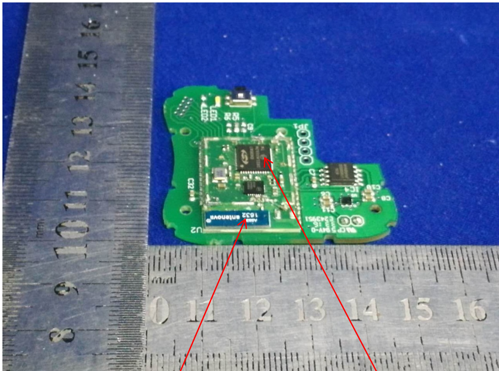
PCB antenna
