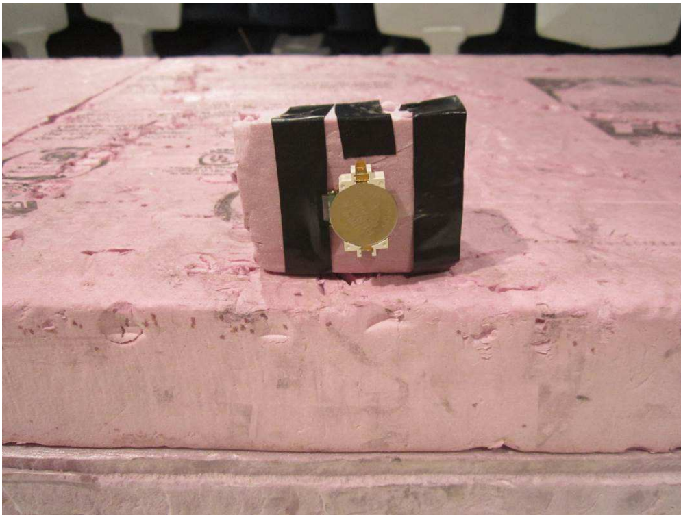
Radiated Emissions – 30 to 1000 MHz (closed up view)
