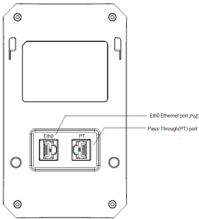
Figure 3 OAW-AP1301H Rear View
