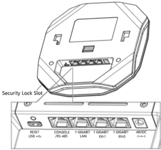
Figure 3: OAW-AP1331 Back View
