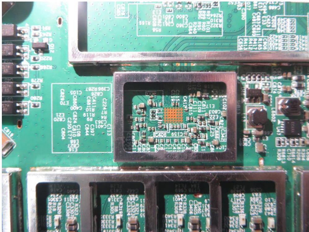
(35) EUT Photo
