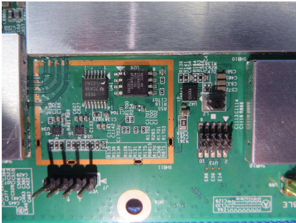
(29) EUT Photo
