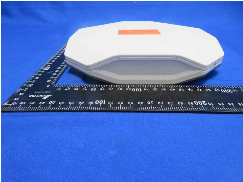
(11) EUT Photo (OAW-AP1411)
