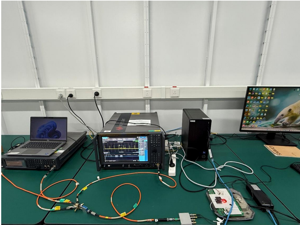
Description: Front View of Conducted Emission Test Setup (Adapter Mode)
