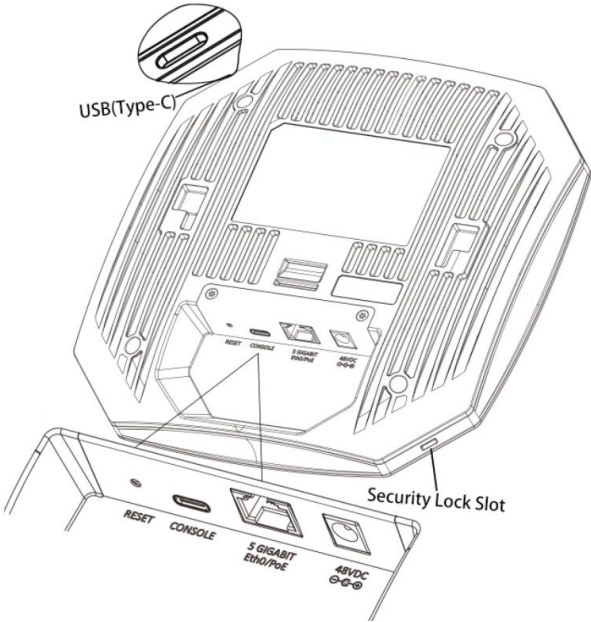
Figure 3: OAW-AP1501 Back View
