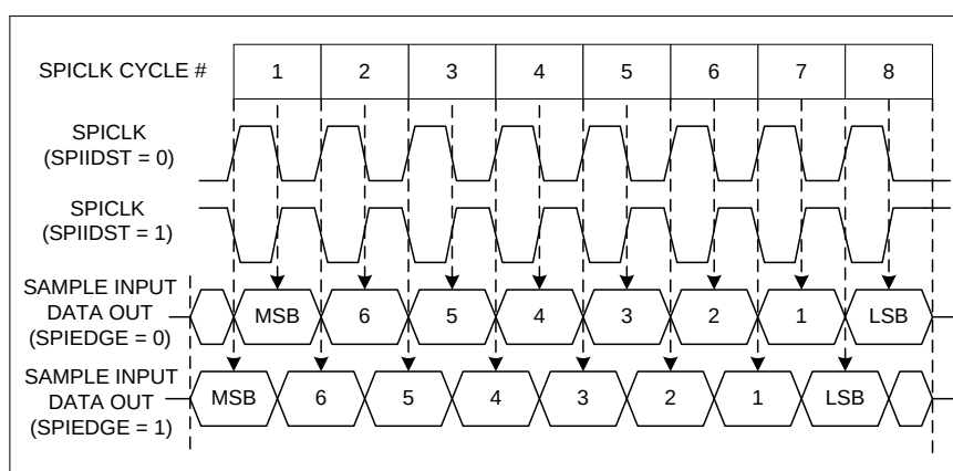
Figure 10-1 SPI timing
