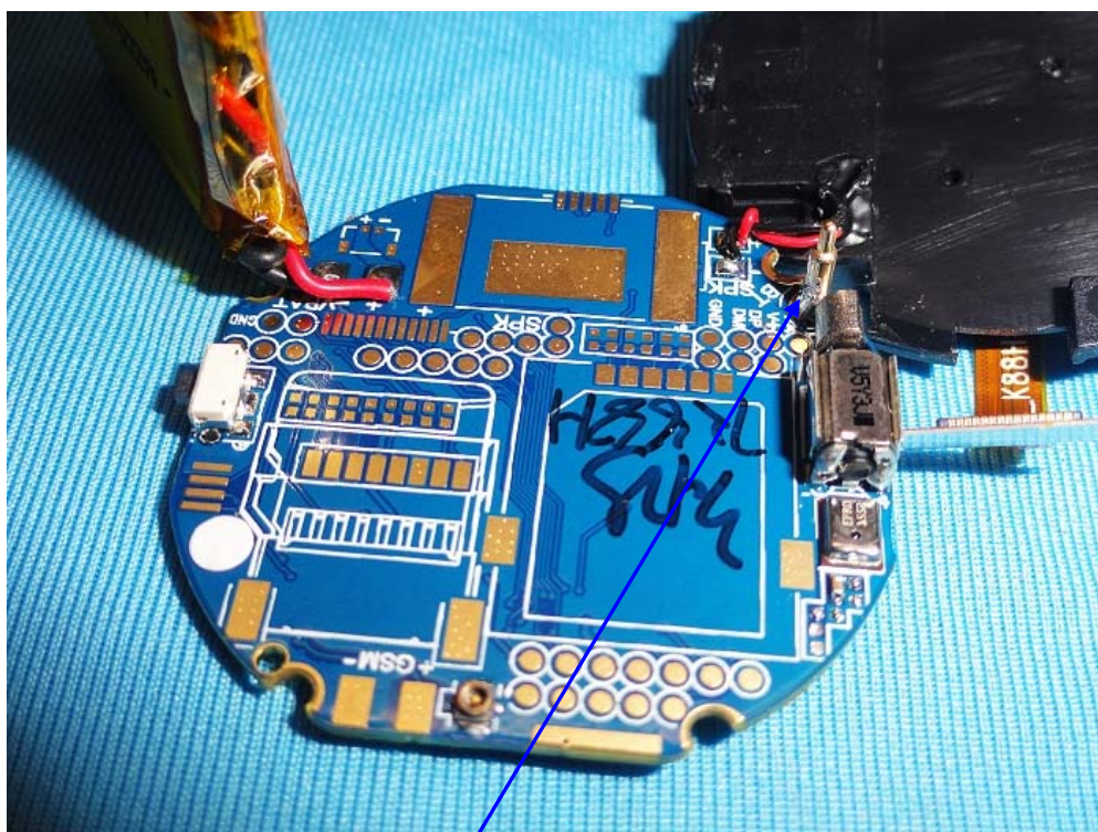
Antenna Connector Pin
