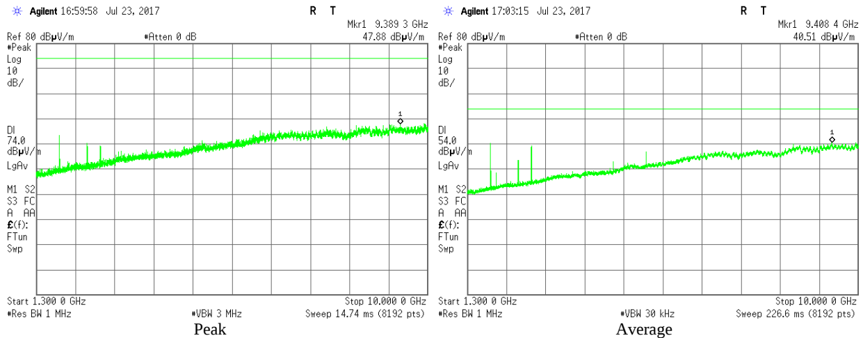
Plot 3.8.27: 3 Radiated Spurious Emission in 1.3 – 10.0 GHz range, Fc =908.6 MHz, BW = 125 kHz SF 10, Vertical
