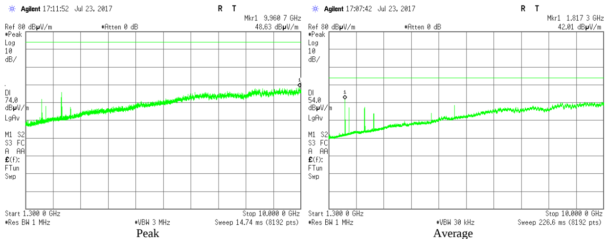
Plot 3.8.28: Radiated Spurious Emission in 1.3 – 10.0 GHz range, Fc =908.6 MHz, BW = 125 kHz SF 10, Horizontal
