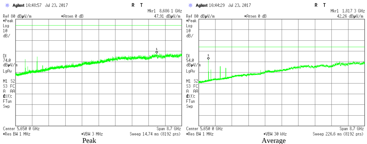
Plot 3.8.16: Radiated Spurious Emission in 1.3 – 10.0 GHz range, F_c = 908.6 MHz, BW = 125 kHz SF 7, Horizontal
