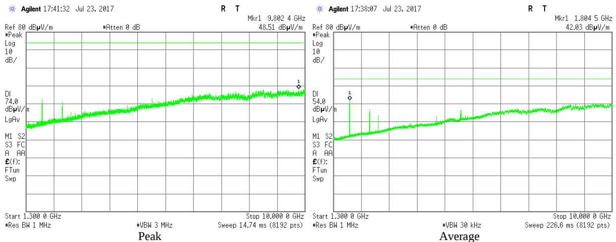
Plot 3.8.24: Radiated Spurious Emission in 1.3 – 10.0 GHz range, F_c = 902.3 MHz, BW = 125 kHz SF 10, Horizontal
