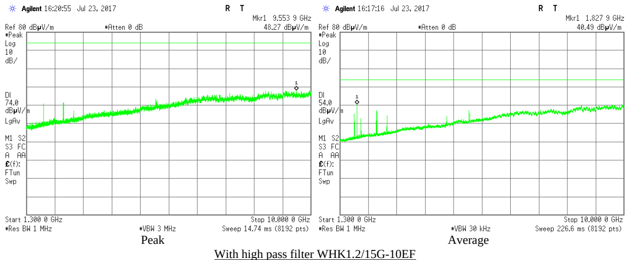
Plot 3.8.44: Radiated Spurious Emission in 1.3 – 10.0 GHz range, F_c = 914.2 MHz, BW = 500 kHz SF8, Horizontal
