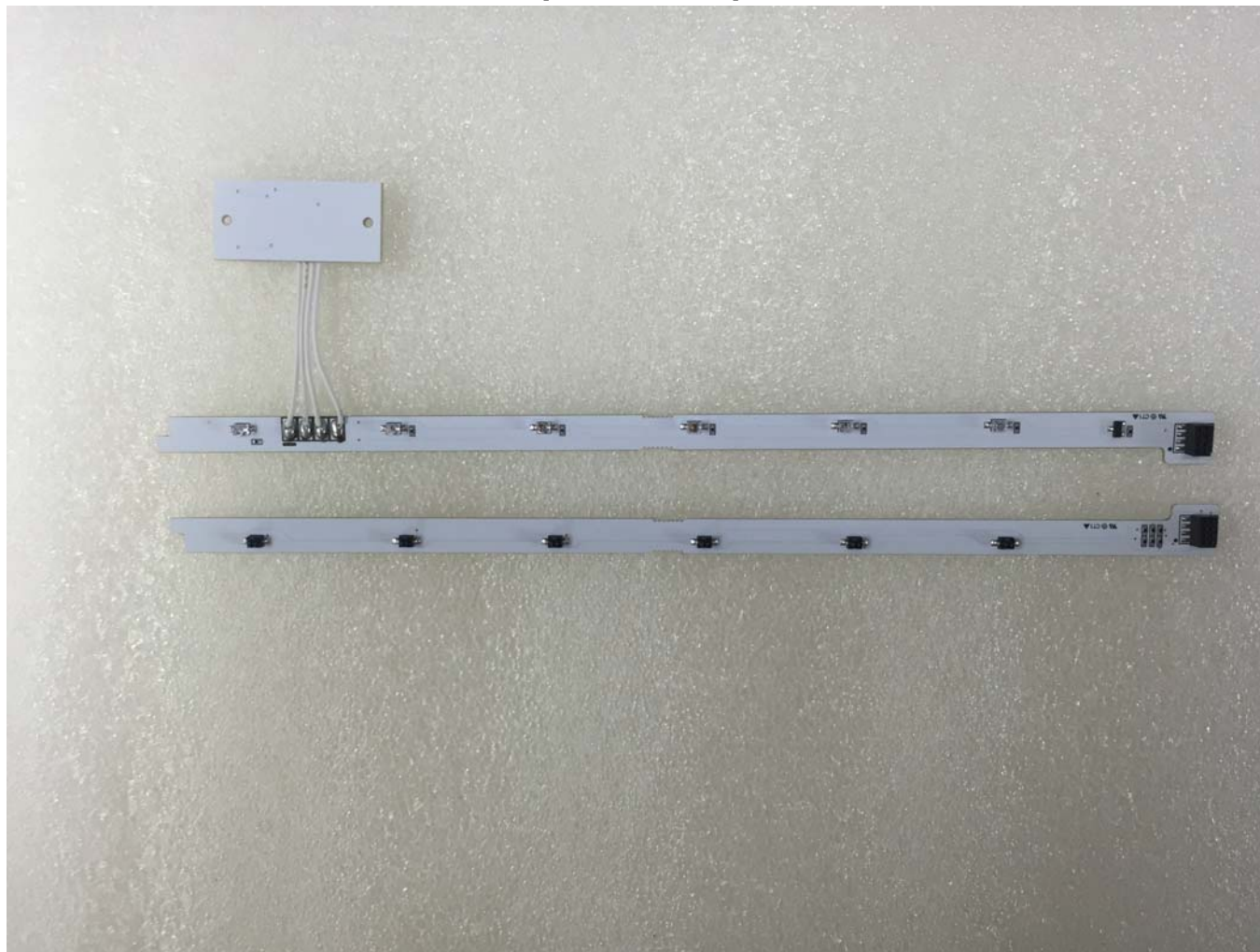
[LED board Front]
