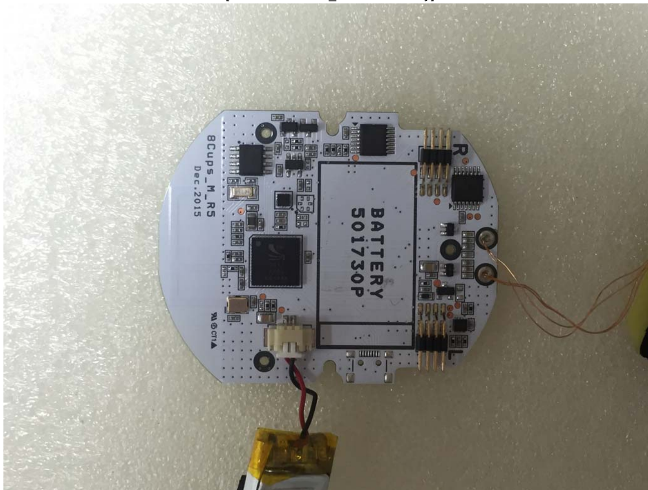
[Main board Front_removed battery]
