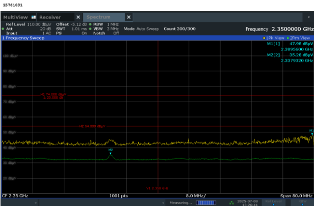
2310 MHz to 2390 MHz Restricted Band
