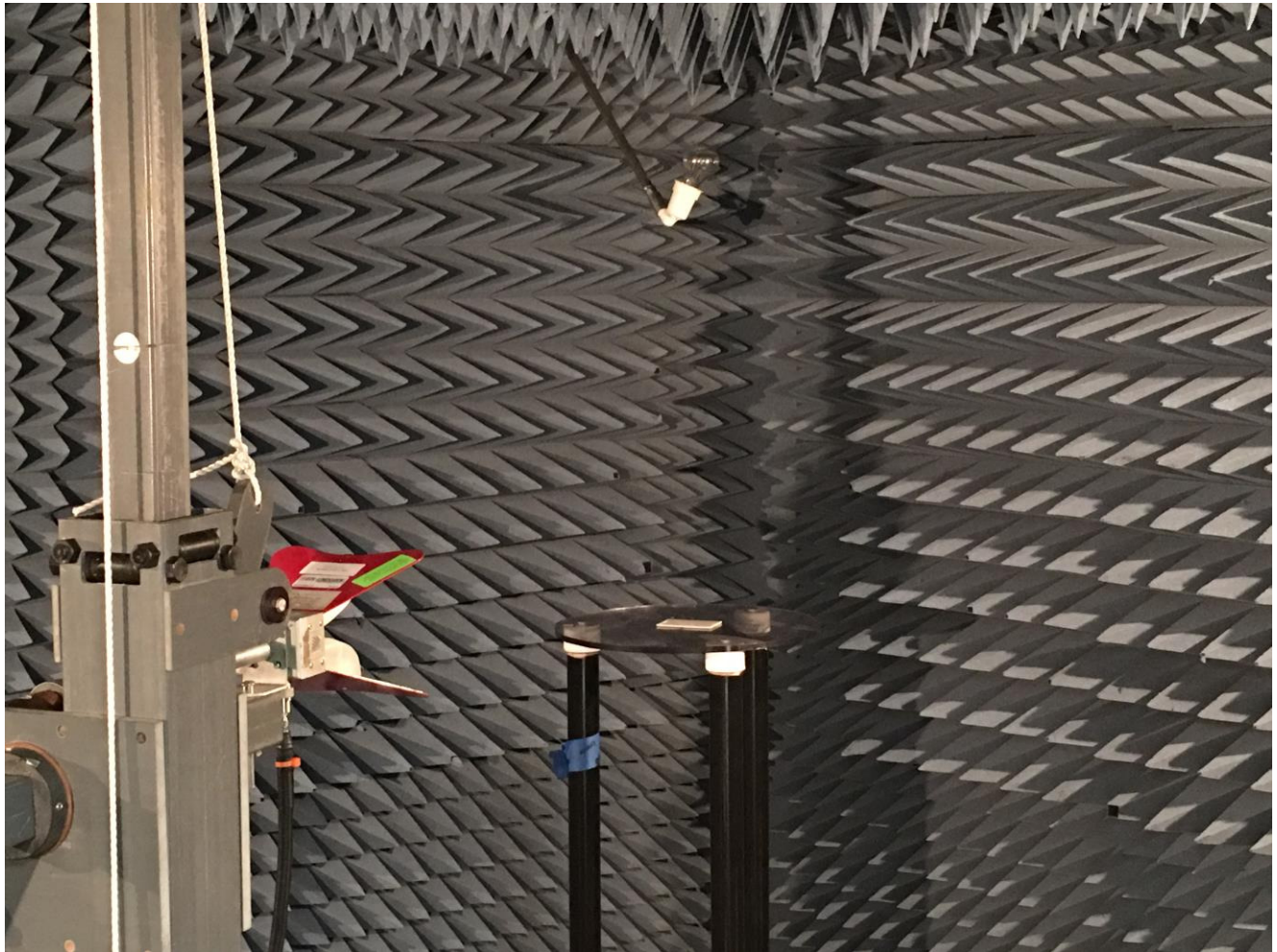
Photograph 2. Radiated Spurious Emissions, Test Setup, Above 1 GHz
