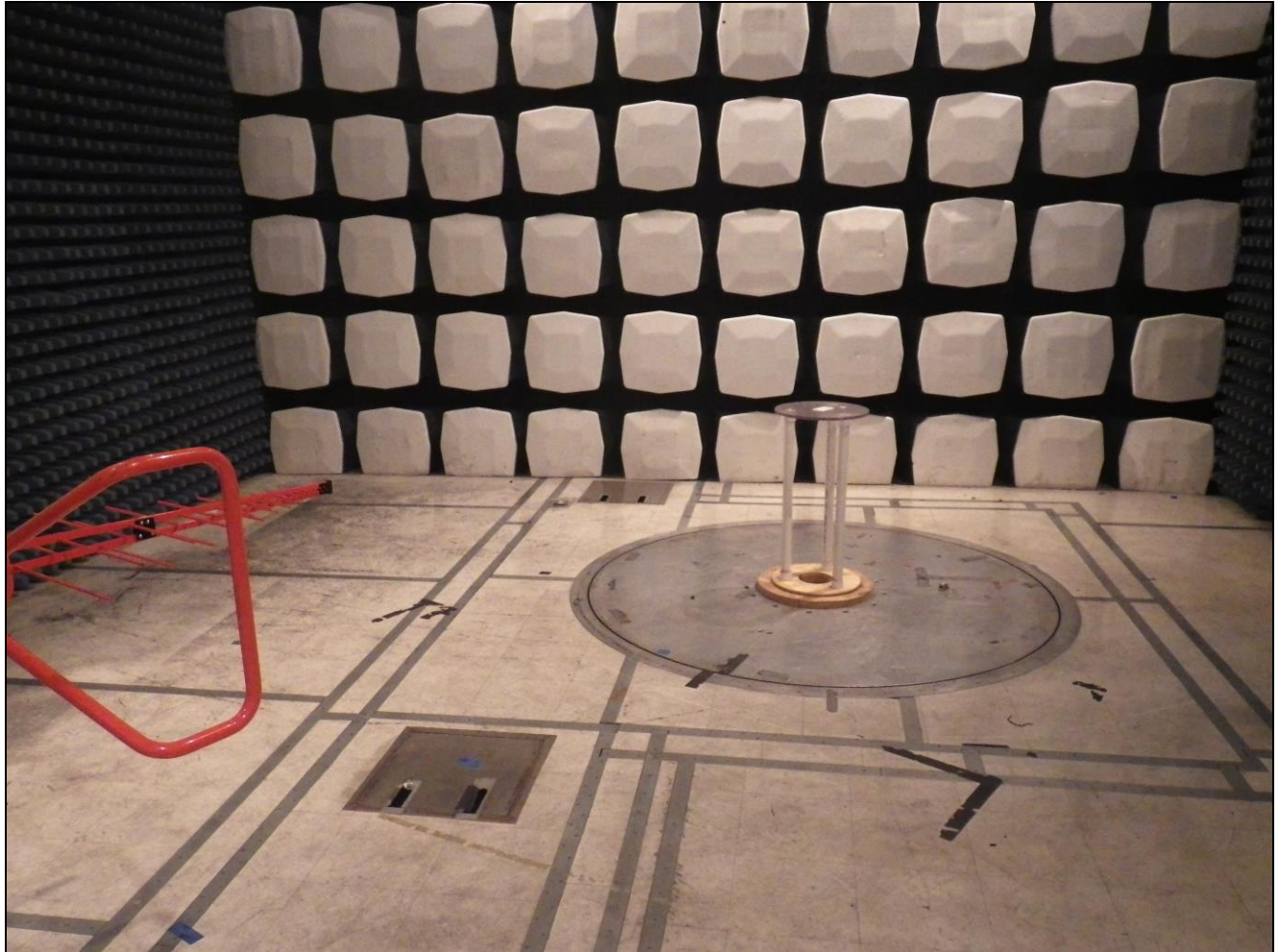
Photograph 1. Radiated Spurious Emissions, Test Setup, Below 1 GHz
