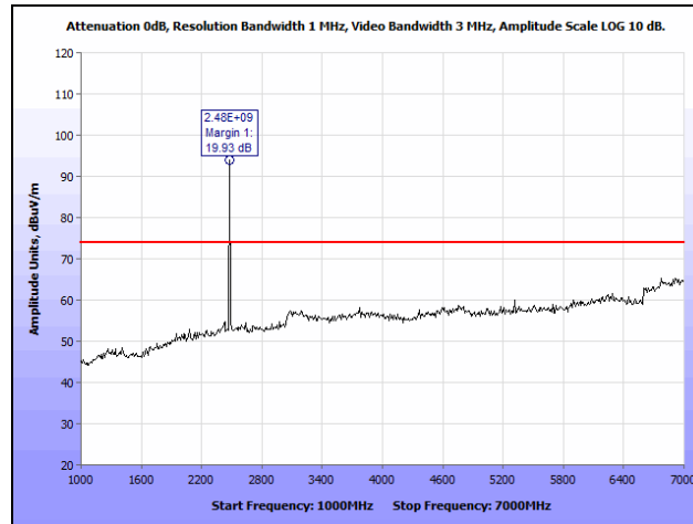
Plot 17. Radiated Spurious Emissions, High Channel, 1 GHz – 7 GHz, Peak
