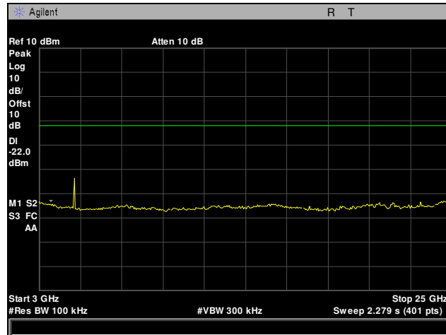
Plot 27. Conducted Spurious Emissions, Mid Channel, 3 GHz – 25 GHz
