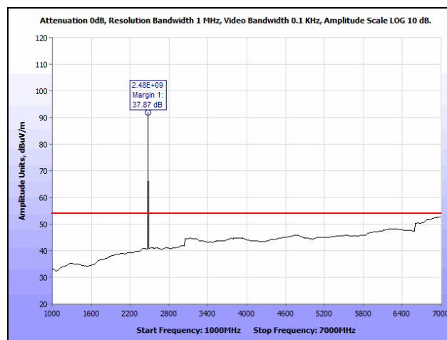
Plot 16. Radiated Spurious Emissions, High Channel, 1 GHz – 7 GHz, Average
