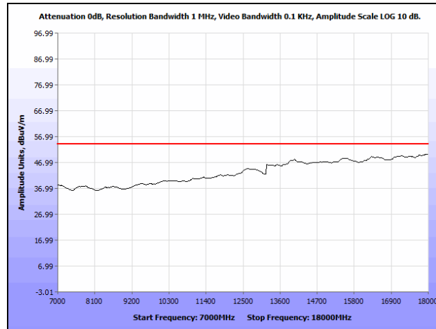
Plot 14. Radiated Spurious Emissions, Mid Channel, 7 GHz – 18 GHz, Average
