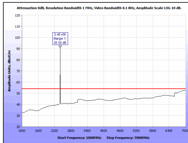
Plot 8. Radiated Spurious Emissions, Low Channel, 1 GHz – 7 GHz, Average
