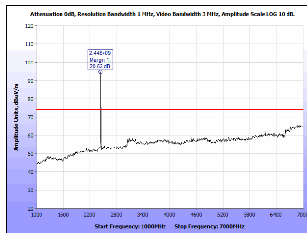
Plot 13. Radiated Spurious Emissions, Mid Channel, 1 GHz – 7 GHz, Peak
