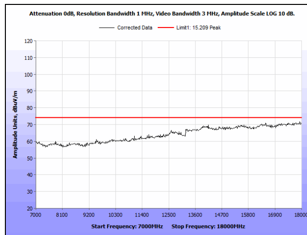
Plot 15. Radiated Spurious Emissions, Mid Channel, 7 GHz – 18 GHz, Peak
