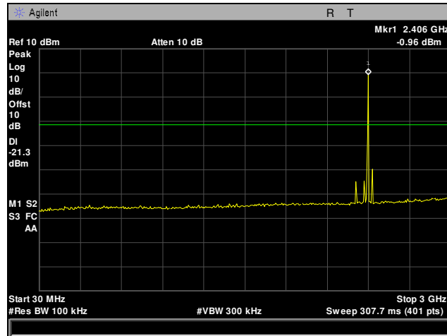
Plot 24. Conducted Spurious Emissions, Low Channel, 30 MHz – 3 GHz
