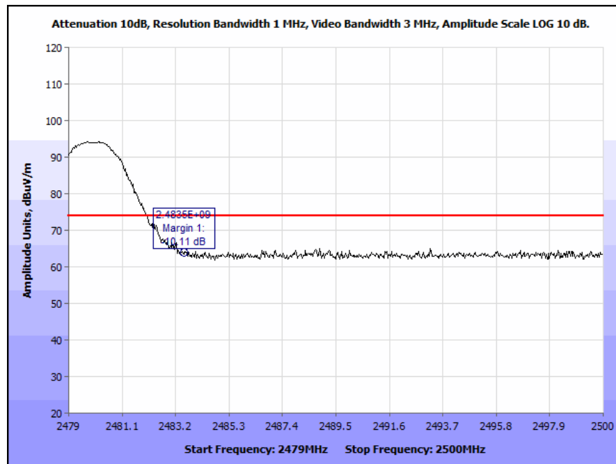
Plot 23. Radiated Restricted Band Edge, High Channel, Peak
