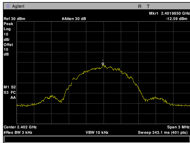
Plot 32. Peak Power Spectral Density, Low Channel
