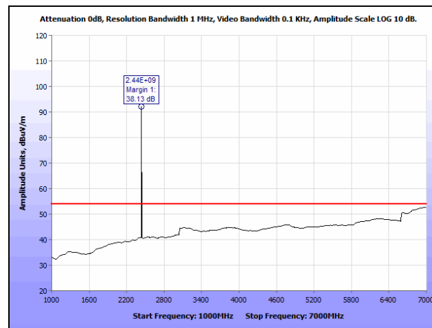
Plot 12. Radiated Spurious Emissions, Mid Channel, 1 GHz – 7 GHz, Average
