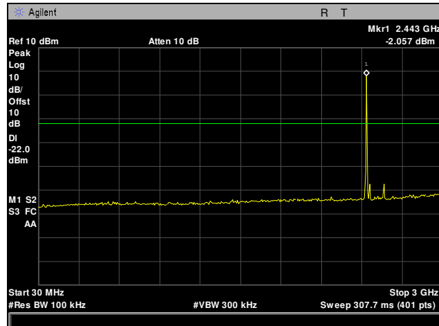
Plot 26. Conducted Spurious Emissions, Mid Channel, 30 MHz – 3 GHz
