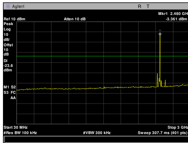
Plot 28. Conducted Spurious Emissions, High Channel, 30 MHz – 3 GHz
