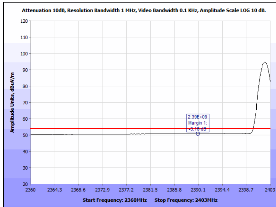
Plot 20. Radiated Restricted Band Edge, Low Channel, Average
