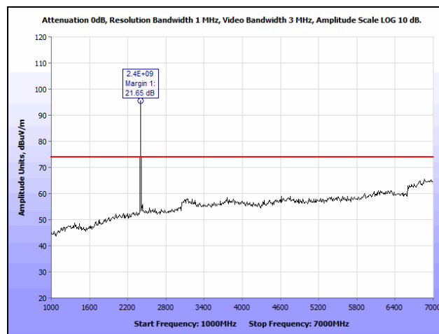
Plot 9. Radiated Spurious Emissions, Low Channel, 1 GHz – 7 GHz, Peak
