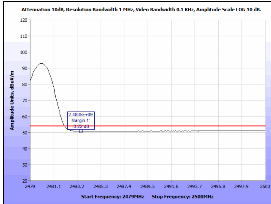
Plot 22. Radiated Restricted Band Edge, High Channel, Average
