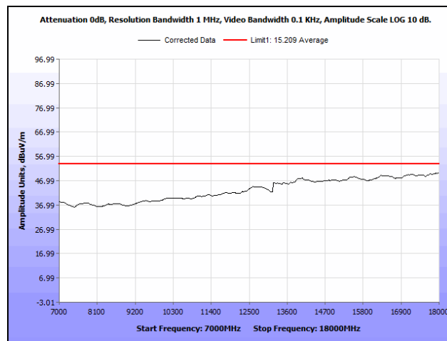
Plot 18. Radiated Spurious Emissions, High Channel, 7 GHz – 18 GHz, Average
