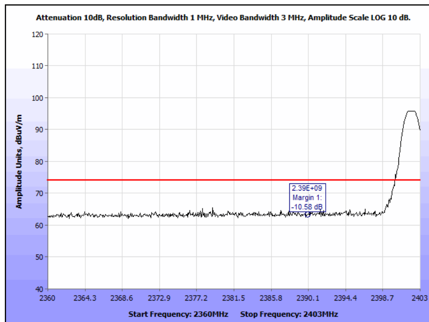
Plot 21. Radiated Restricted Band Edge, Low Channel, Peak
