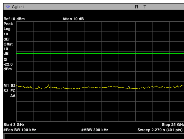
Plot 29. Conducted Spurious Emissions, High Channel, 3 GHz – 25 GHz
