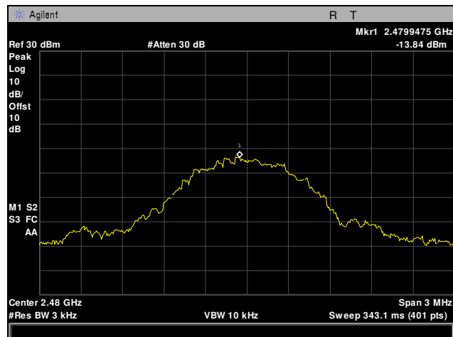
Plot 34. Peak Power Spectral Density, High Channel
