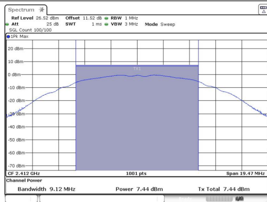
Conducted Output Power IEEE 802.11b_Channel 1_Antenna 0
