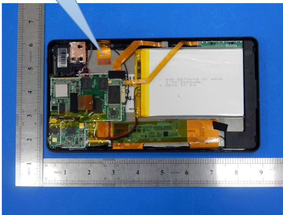
BT&WIFI Antenna location
