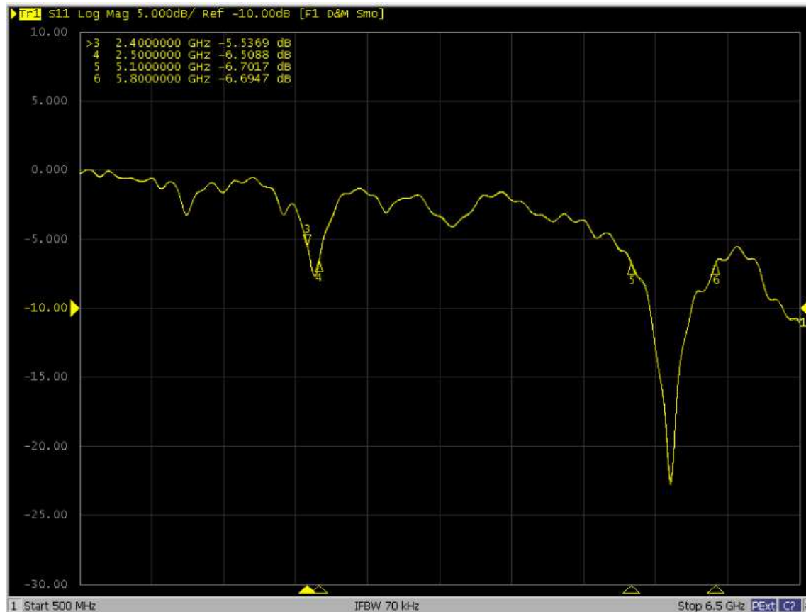
Ant2_S11
