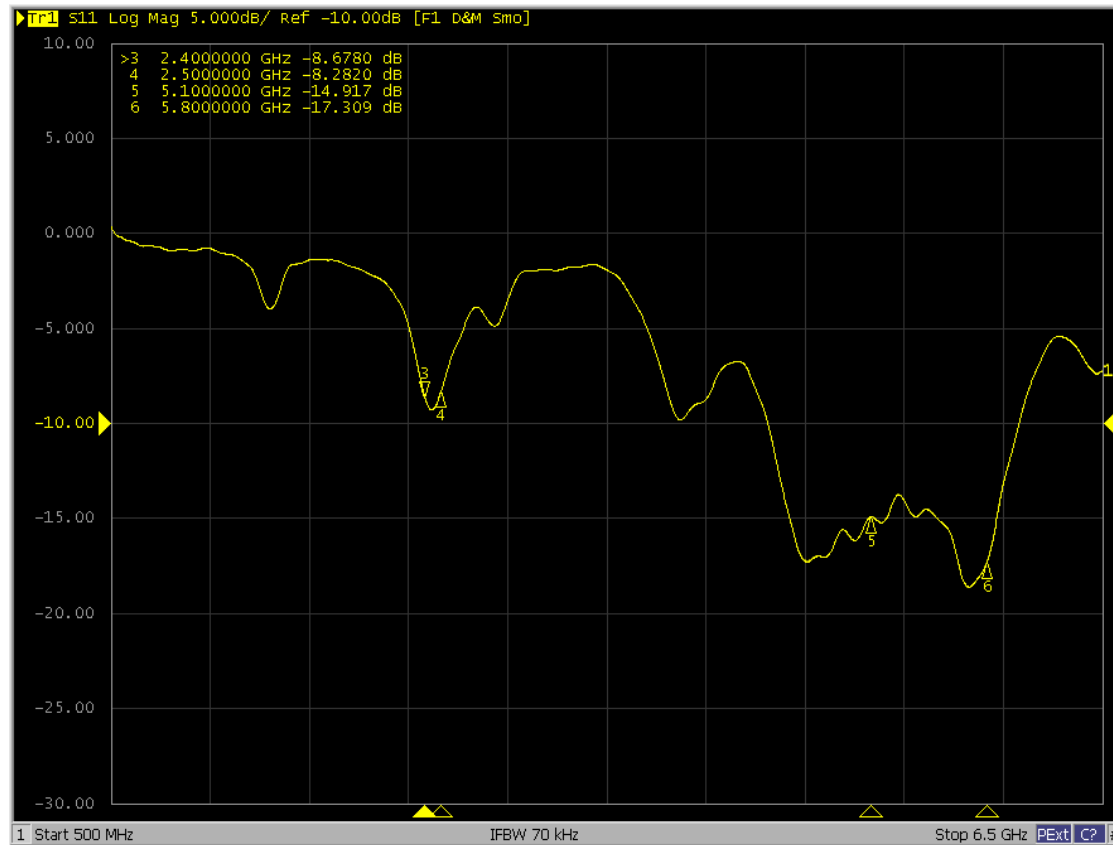
Ant1_S11
