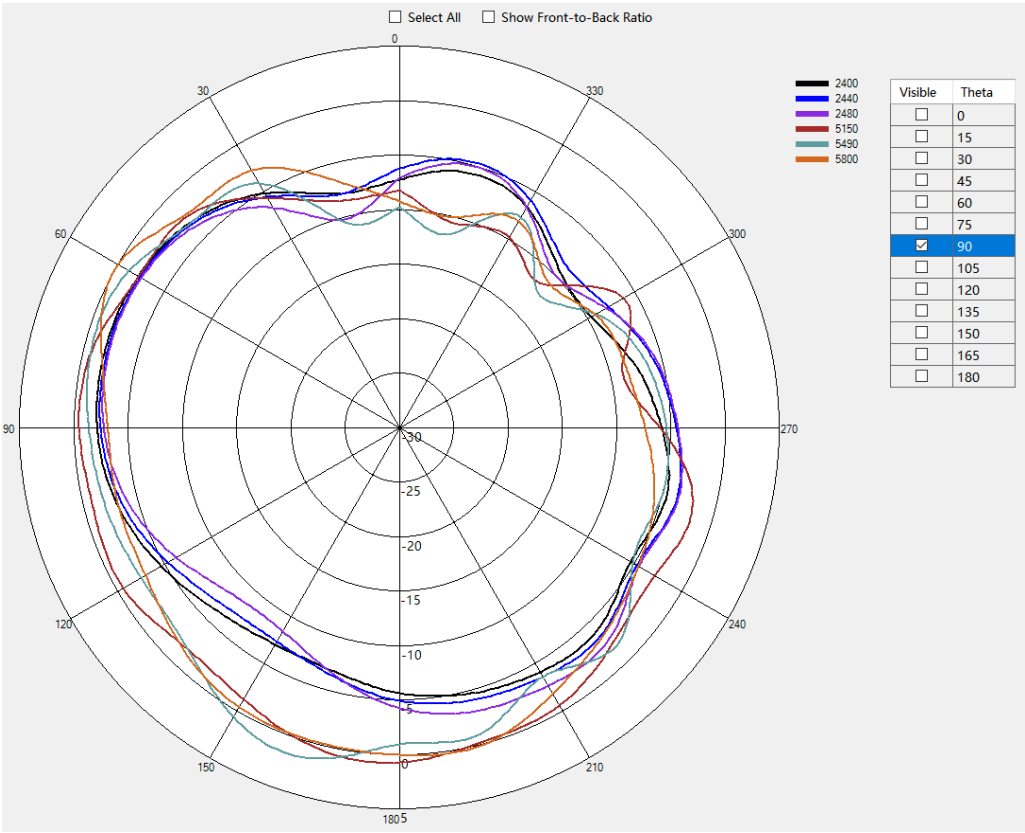
Ant1_2D_Theta90°
