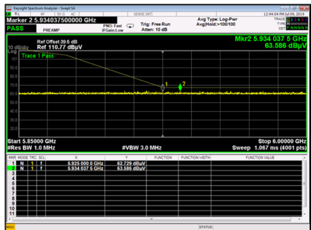
Band IV 11n20 CH165 Peak
