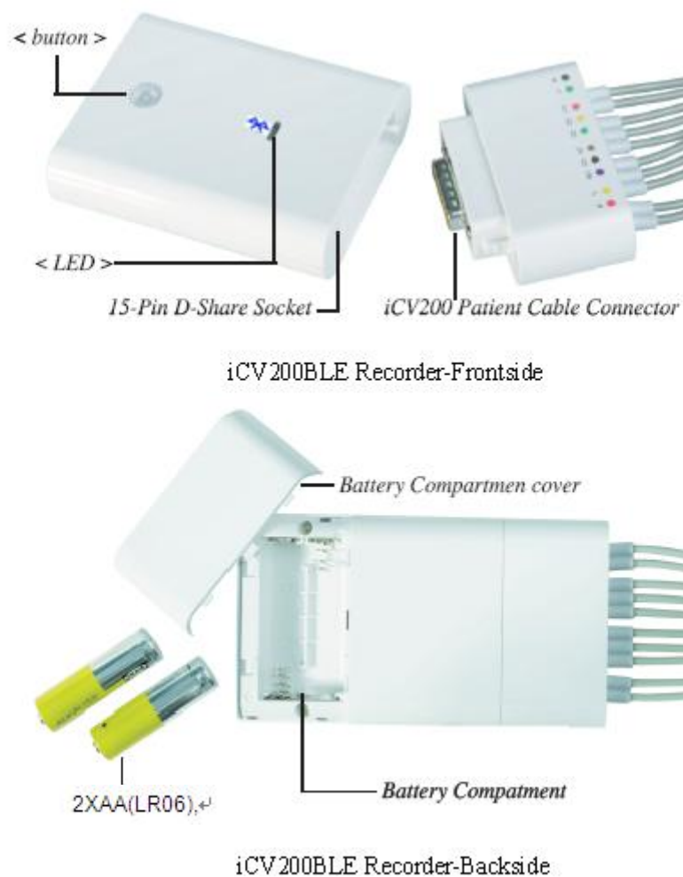
Fig 2.1 iCV200(BLE) Recorder
