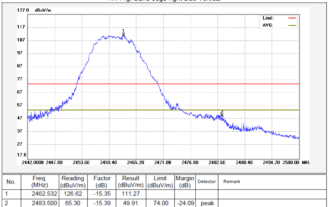
TX 11g: Band edge-right side Vertical
