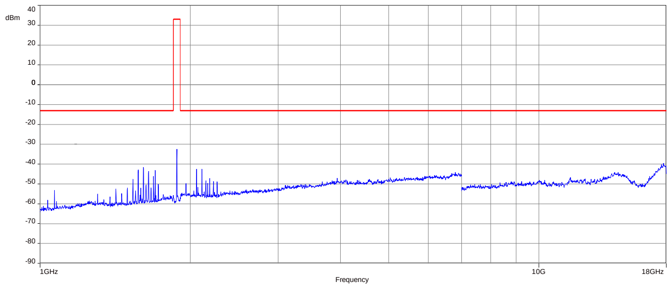
Plot 3: Mid channel (1 GHz – 18 GHz)
