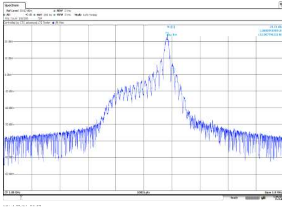
Plot 21: mid channel (99% - OBW), spacing 15 kHz, 1@11 tones
