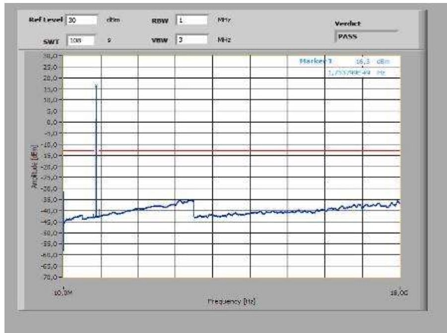
Plot 15: Highest Channel (10 MHz – 18 GHz), spacing 15 kHz, 12@0 tones
