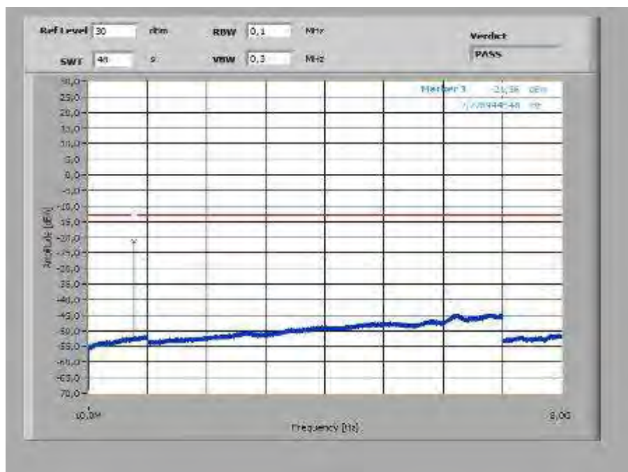
Plot 15: Highest Channel (10 MHz – 8 GHz), spacing 15 kHz, 12@0 tones
