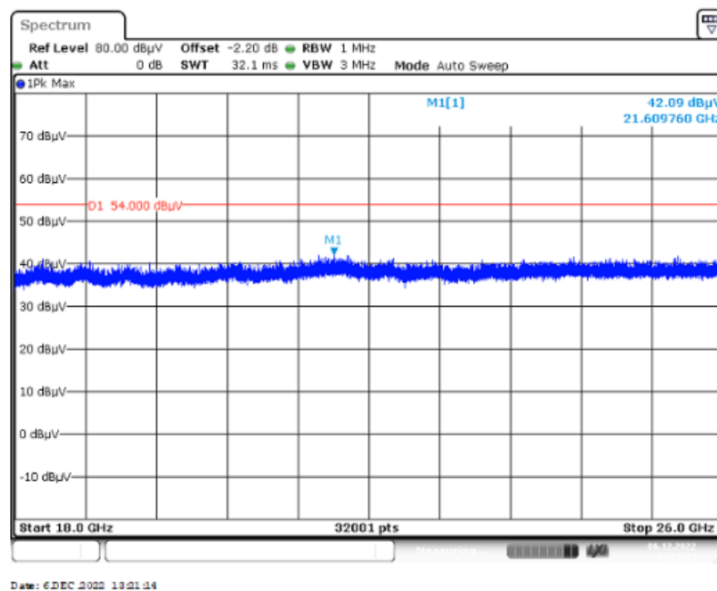
Plot 4: 18 GHz to 26 GHz, vertical & horizontal polarization, 1 Msps, valid for all channels
