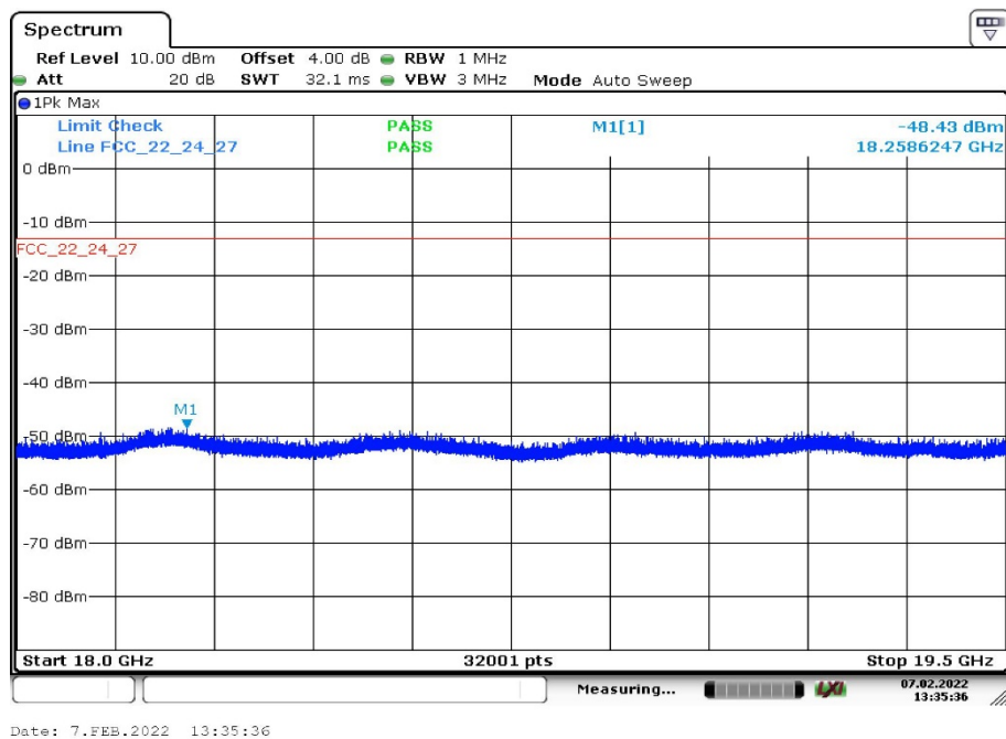
Plot 4: Channel 661 (18 GHz – 19.5 GHz)
