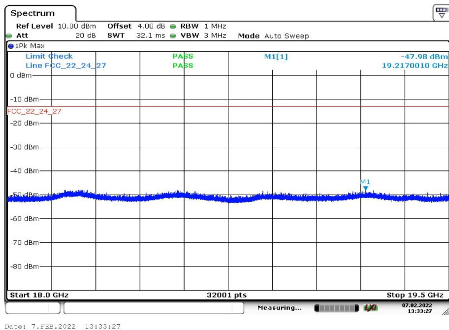
Plot 3: Channel 661 (18 GHz – 19.5 GHz)
