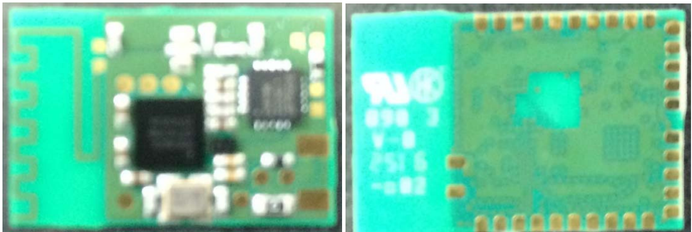
Figure 2 - Owlet Wearable Sensor – Radio PWB – Front and Back Side
