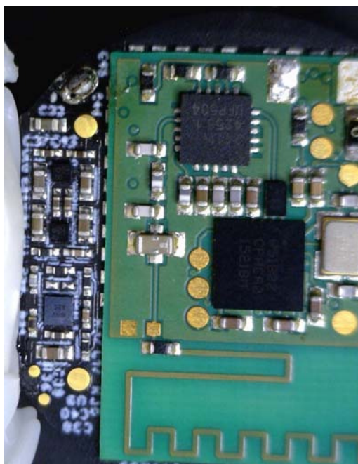
Figure 5 - Owlet Wearable Sensor RF section
