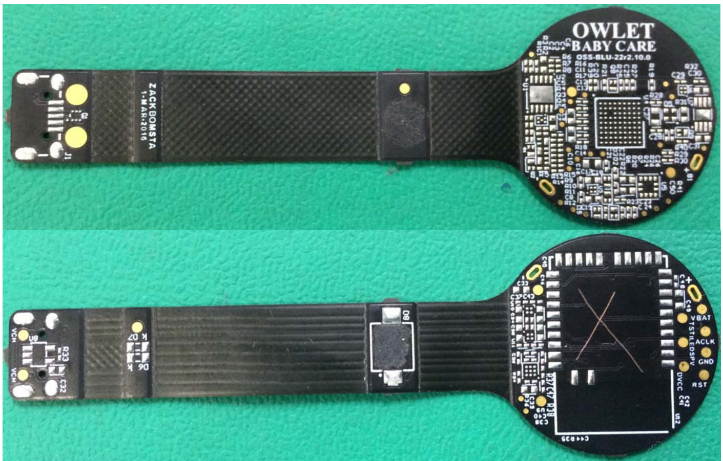
Figure 3 - Owlet Wearable Sensor – Main PWB w/o Radio PWB – Front and Back Side
