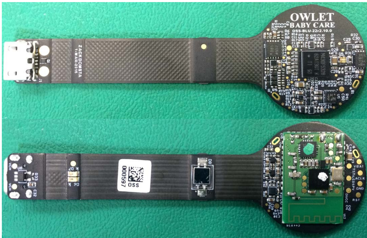
Figure 4 - Owlet Wearable Sensor – Main PWB w/ Radio PWB – Front and Back Side
