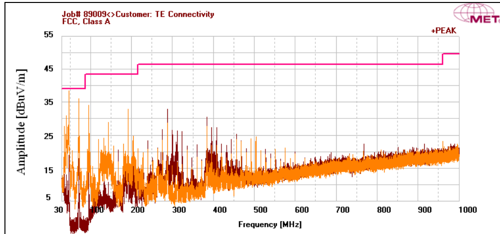
Plot 12. Radiated Spurious Emissions, Mid Channel, 30 MHz – 1 GHz
