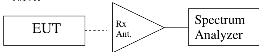
Figure 5. Block Diagram, Peak Power Spectral Density Test Setup
