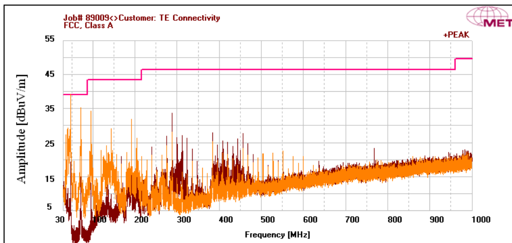
Plot 9. Radiated Spurious Emissions, Low Channel, 30 MHz – 1 GHz
