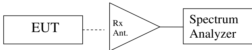
Figure 4. Block Diagram, Conducted Spurious Emissions Test Setup
