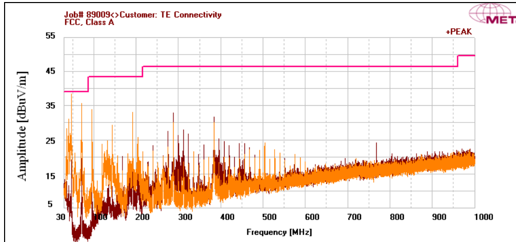
Plot 15. Radiated Spurious Emissions, High Channel, 30 MHz – 1 GHz
