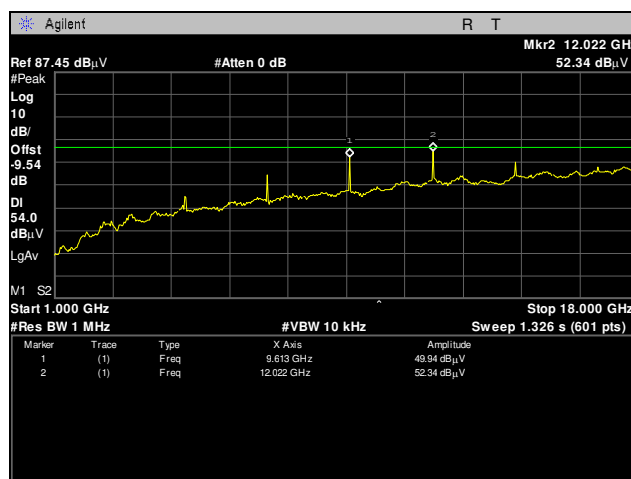
Plot 10. Radiated Spurious Emissions, Low Channel, 1 GHz – 18 GHz, Average
