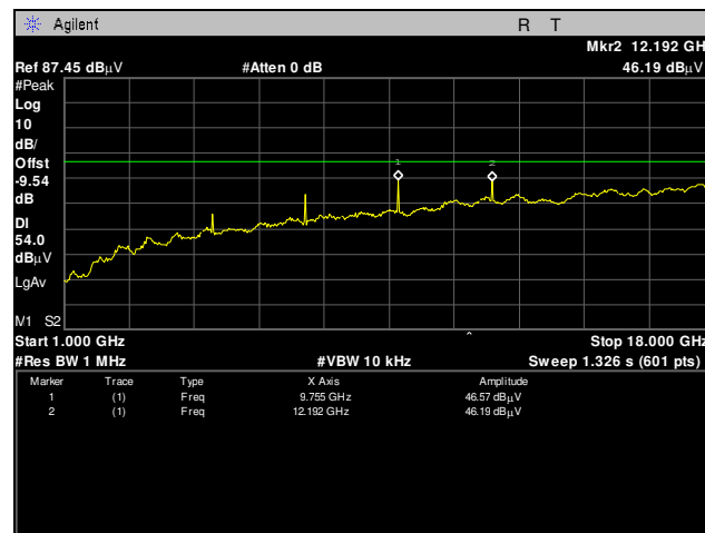
Plot 13. Radiated Spurious Emissions, Mid Channel, 1 GHz – 18 GHz, Average
