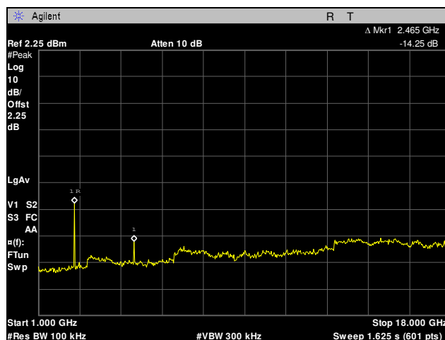
Plot 27. Conducted Spurious Emissions, High Channel, 1 GHz – 18 GHz
