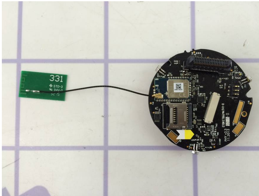
Antenna view
