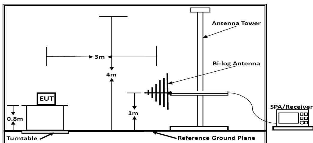
Below 1GHz
