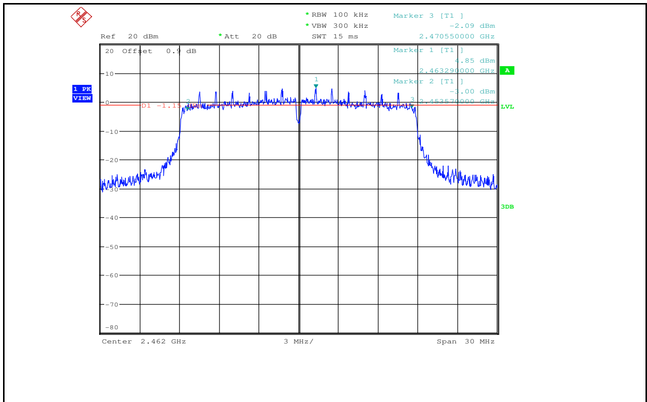
6dB Bandwidth_11N20ISO_2462_Ant2
