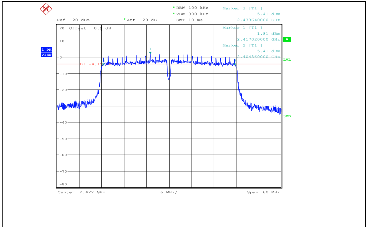
6dB Bandwidth_11N40ISO_2422_Ant2
