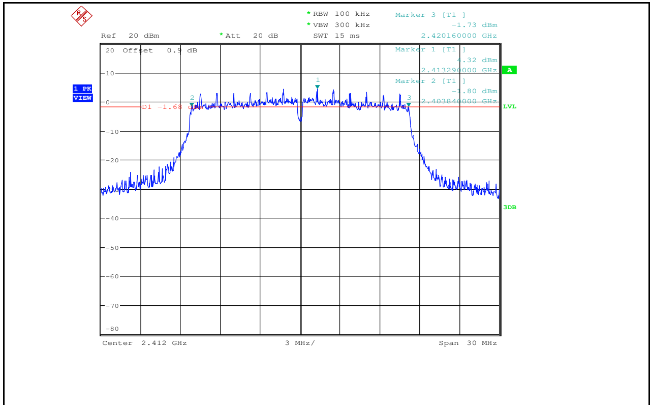
6dB Bandwidth_11G_2412_Ant2
