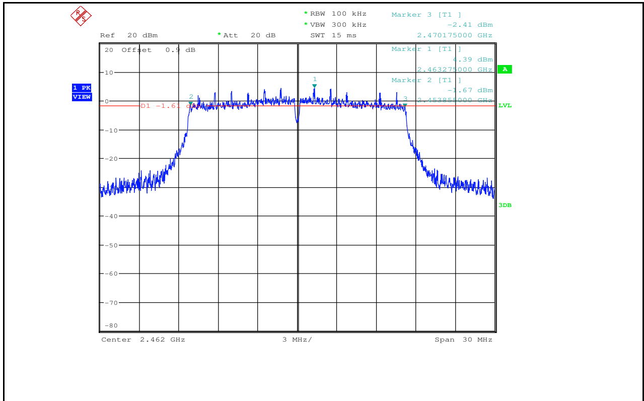
6dB Bandwidth_11G_2462_Ant2
