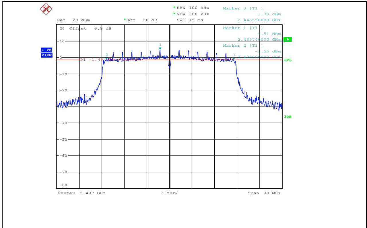
6dB Bandwidth_11N20SISO_2437_Ant2
