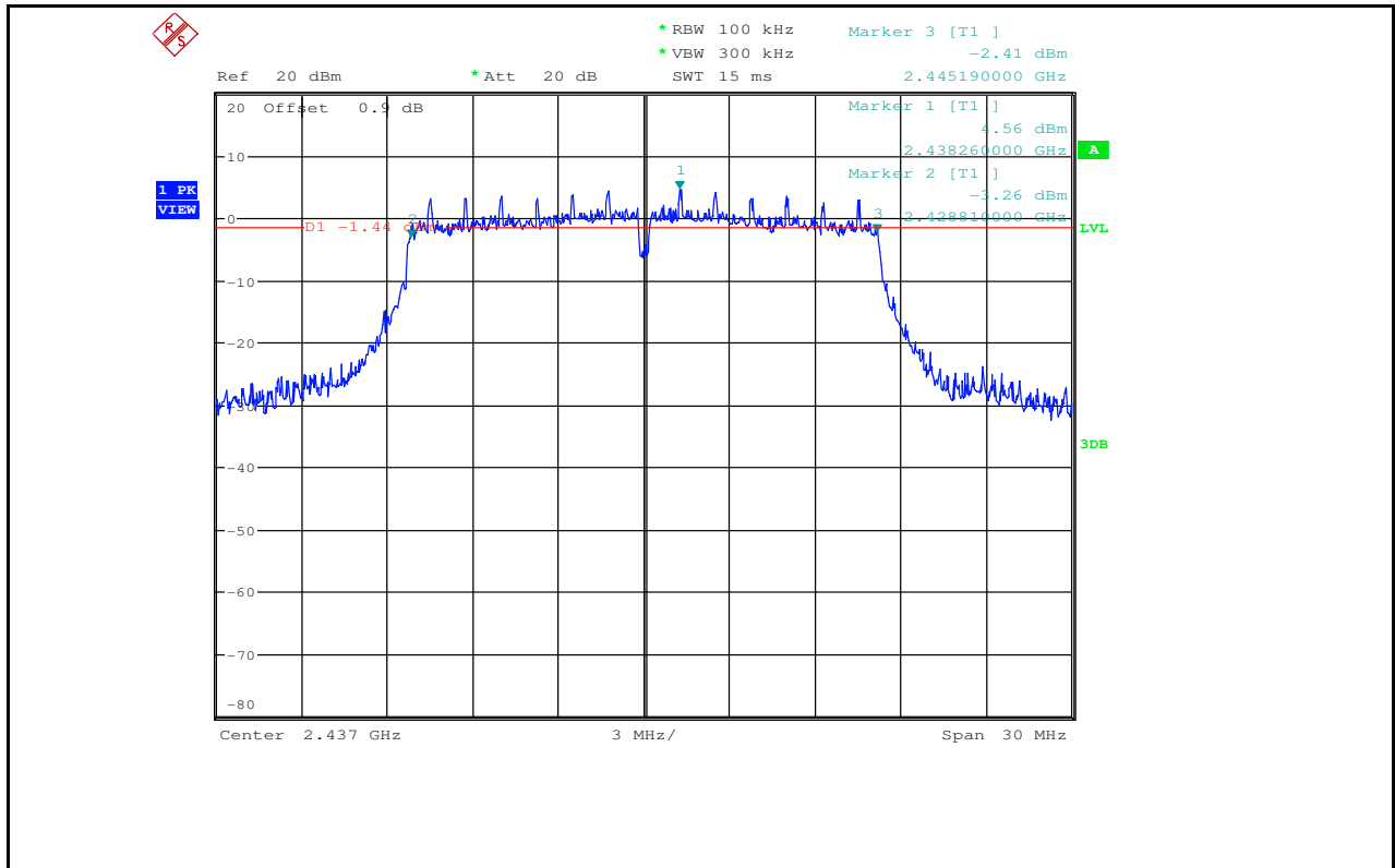
6dB Bandwidth_11G_2437_Ant2
