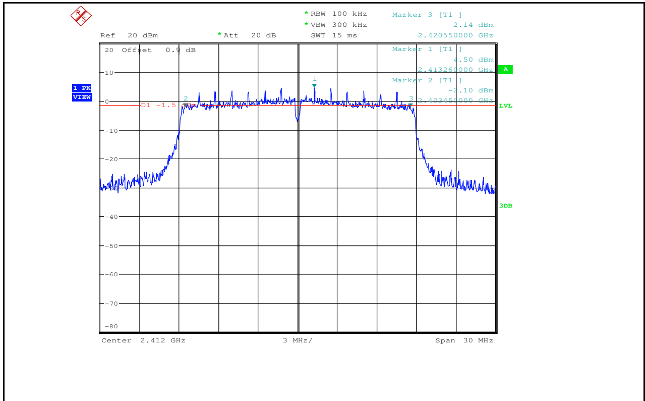
6dB Bandwidth_11N20SISO_2412_Ant2
