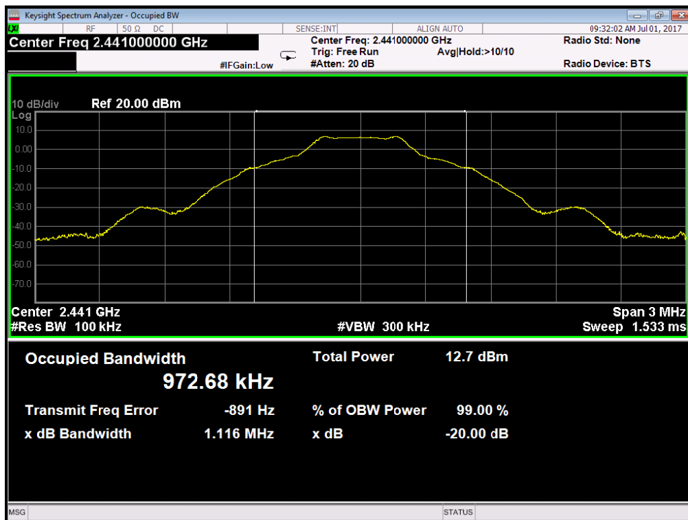
39 Channel @ GFSK
