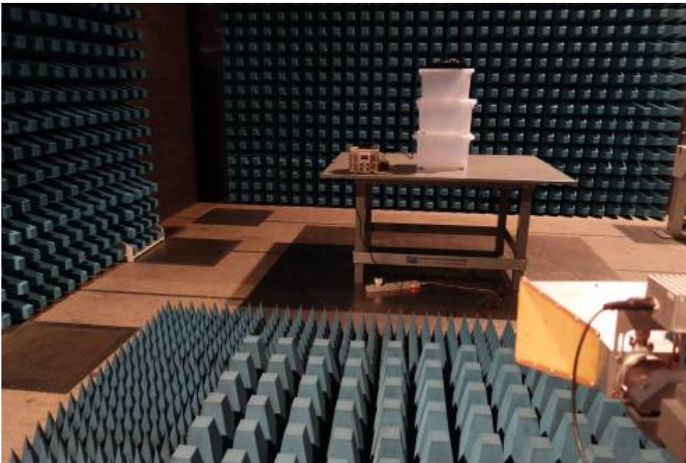
Re ( Above1GHz )
